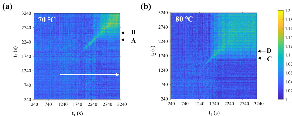
Fig. 2 Two-time correlation function C_1 for q_{\parallel} = 1.78 \times 10^{-3} \text{ nm}^{-1} at 70 °C (a) and 80 °C (b). The correlation function at a specific time can be evaluated by cutting out horizontally as shown by the white arrow. Arrows A and B in (a) correspond to t_w = 2320 and 2540 s, respectively, and arrows C and D in (b) correspond to t_w = 1620 and 1890 s, respectively.
