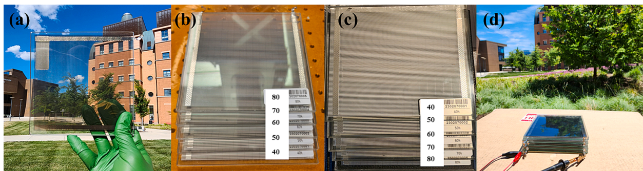
Fig. 3. Photographs of (a) 80% CdTe solar panel on campus; (b) five CdTe solar panels stacked in parallel with descending transparency: 80%,70%,60%,50%, 40%, (c) five CdTe solar panels stacked in parallel with ascending transparency: 40%,50%,60%,70%, 80%, (d) I-V measurement set for five CdTe solar panels stacked in parallel (experimental date: June 26, 2023, location: outside of Rhodes Hall on the main campus of University of Cincinnati).
