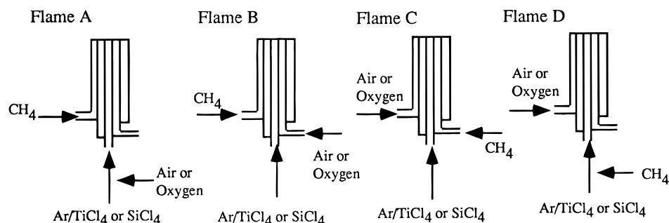
Figure 1. Reactant gas mixing configurations for diffusion reactors. 15
