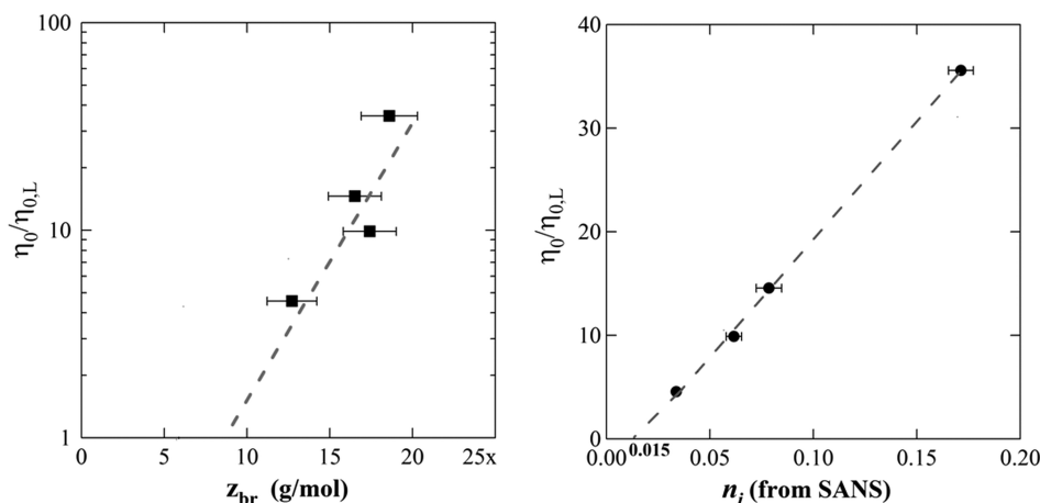
Figure 4. (a, left) Log-linear plot of zero shear rate viscosity enhancement for linear polyethylene of the same M_w^{22} against the average length of a branch, z_{br} (from SANS), for the HDB samples. The extrapolation of z_{br} data intercepts the z_{br} axis at 9000 g/mol. (b, right) Linear plot of zero shear rate viscosity enhancement for linear polyethylene of same M_w^{22} against number of inner segments per chain, n_i , for the HDB samples. The error in n_i for HDB-1 is smaller than the point size.
