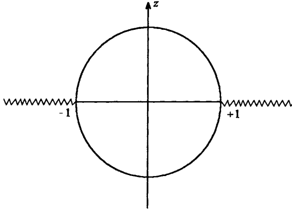
Fig. 13.7 For the \frac{1}{\sqrt{z^2-1}} function we write the Taylor series in the region |z| < 1
