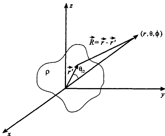
Fig. 11.9 Multipole expansion
