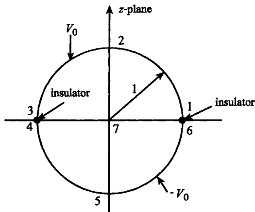
Fig. 12.15 Two conductors with semicircular cross sections
