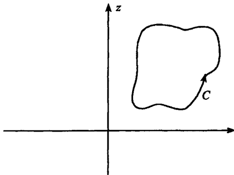
Fig. 13.1 Contour for the Cauchy-Goursat theorem
