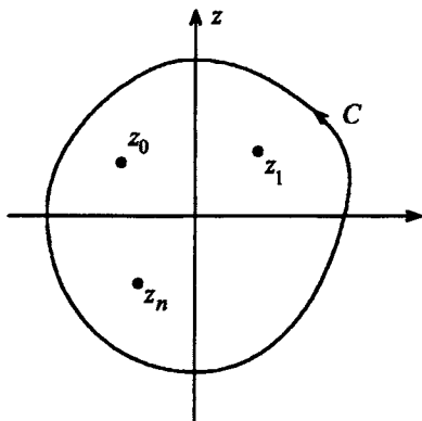
Fig. 13.9 Residue theorem
