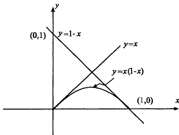
Fig. 17.4 \sin(\pi x) could be approximated by x(1-x)
