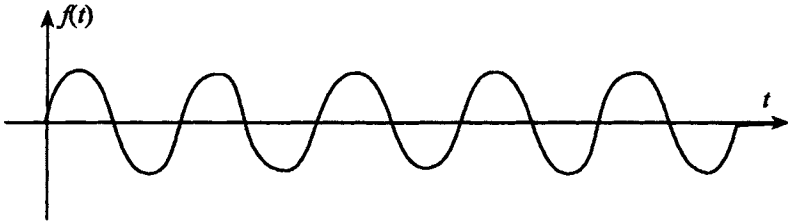
Fig. 16.1 Wave train with N = 5
