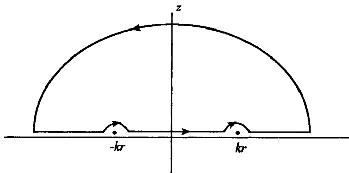
Fig. 13.20 Contour for I_1
