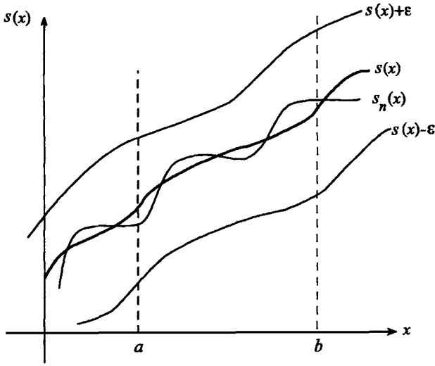
Fig. 15.2 Uniform convergence is very important
