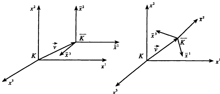
Fig. 11.3 Boost and boost plus rotation
