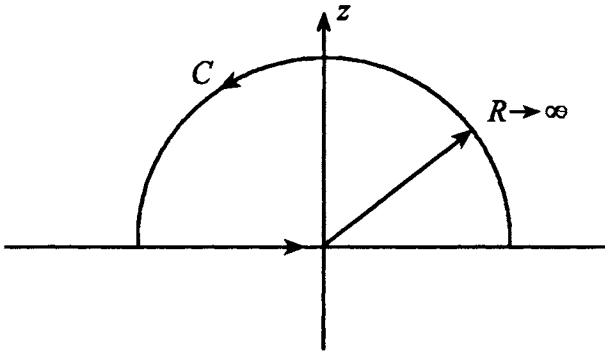
Fig. 13.13 Contour for the type II integrals
