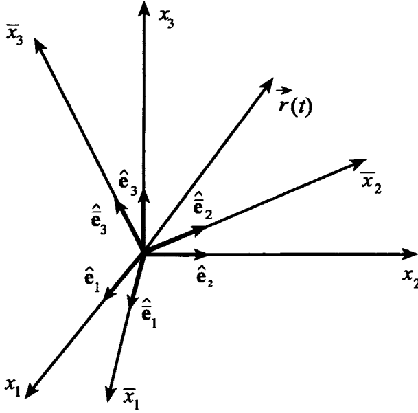
Fig. 10.4 Direction cosines
