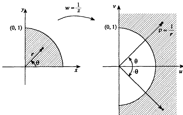
Fig. 12.4 Inversion maps circles to circles
