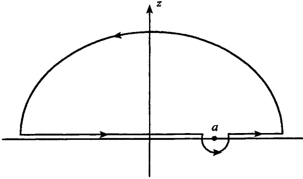
Fig. 13.19 Another path for the Cauchy principal value calculation
