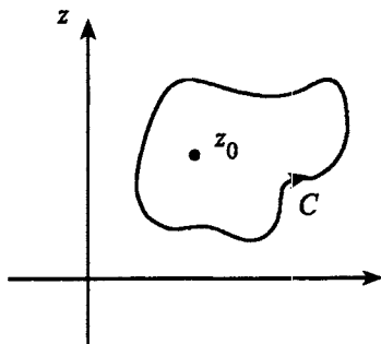
Fig. 13.2 Contour for the Cauchy integral theorem
