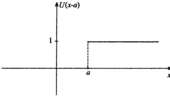
Fig. 16.4 Heaviside step function
