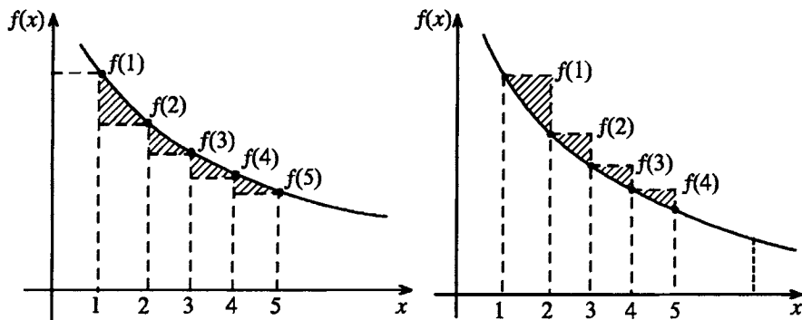
Fig. 15.1 Integral test
