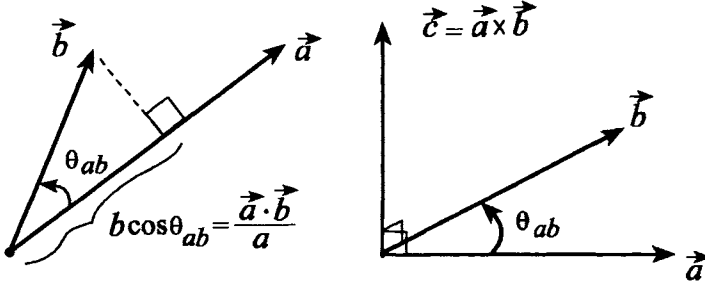
Fig. 10.2 Scalar and vector products
