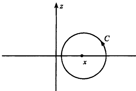
Fig. 13.22 Contour for the Schlöfli formula
