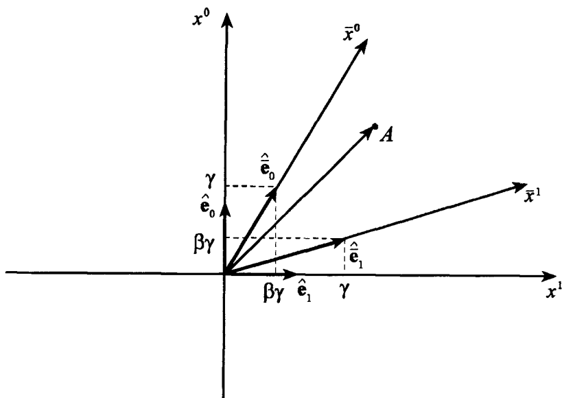
Fig. 10.11 Orientation of the \overline{K} axis with respect to the K frame
