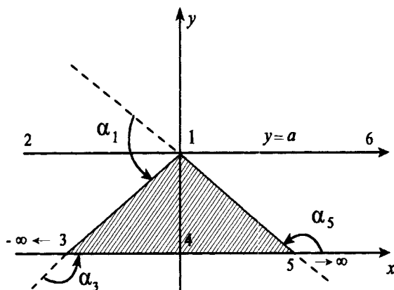
Fig. 12.31 Triangular region
