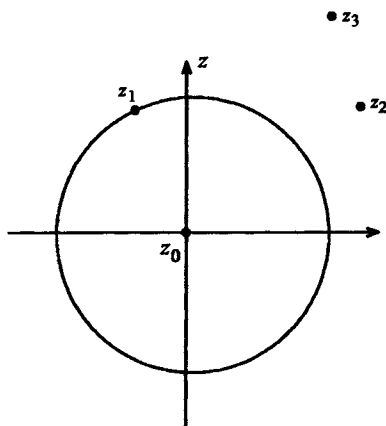
Fig. 13.11 Analytic continuation
