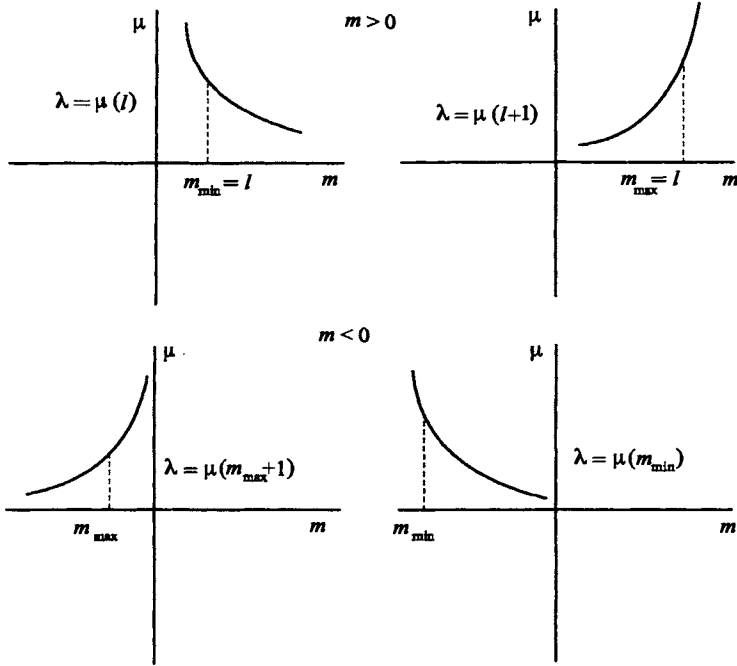
Fig. 9.1 Different cases for \mu(m)
