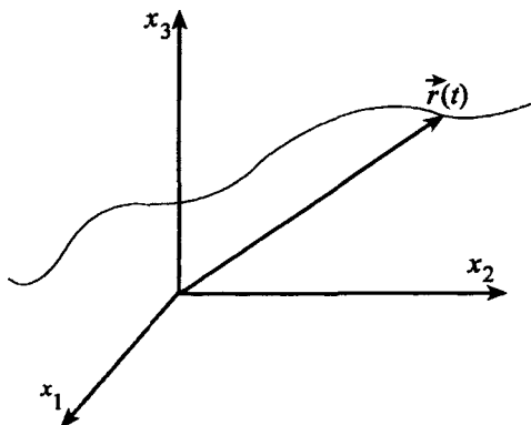
Fig. 10.3 Motion in Cartesian coordinates
