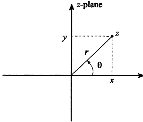
Fig. 12.1 A point in the complex z -plane
