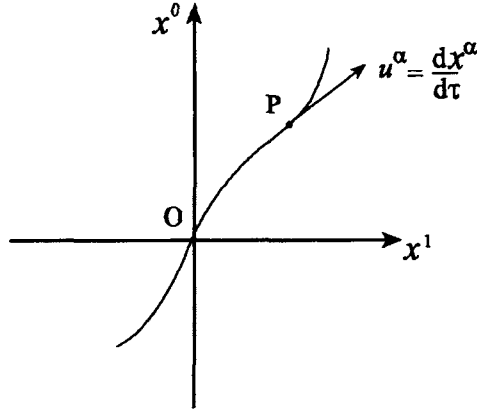
Fig. 10.10 Worldlines and four-velocity
