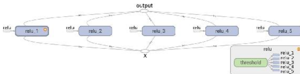
Figure 9-8. Five ReLUs sharing the threshold variable
