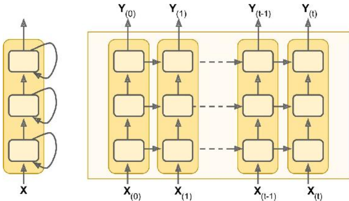
Figure 14-12. Deep RNN (left), unrolled through time (right)
