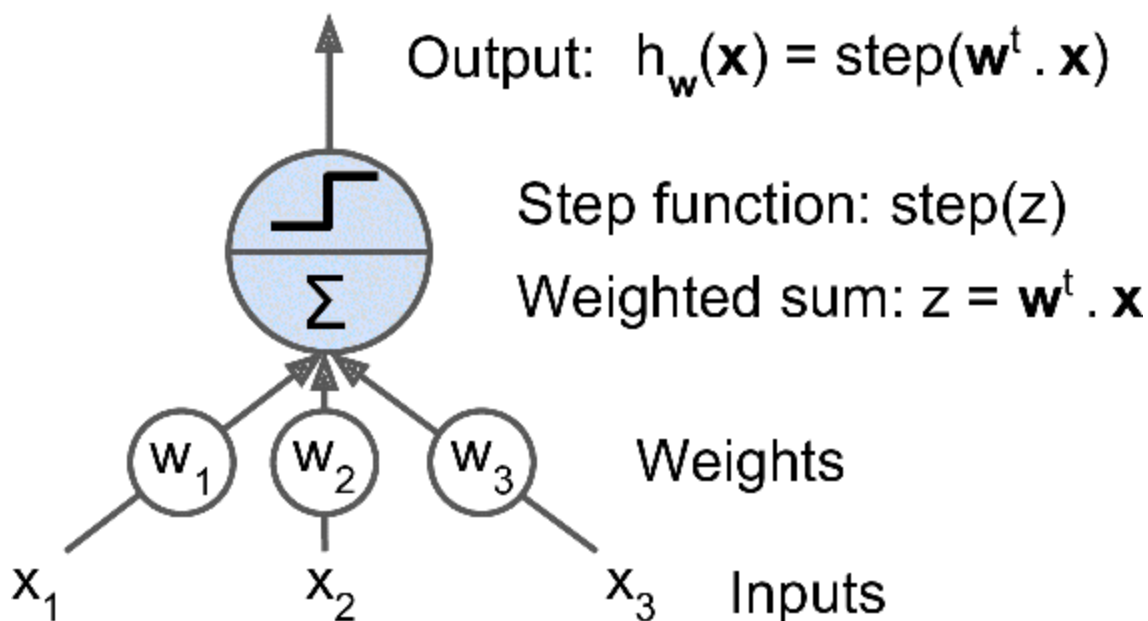
Figure 10-4. Linear threshold unit
