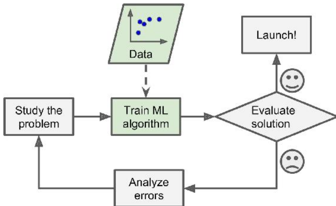
Figure 1-2. Machine Learning approach
