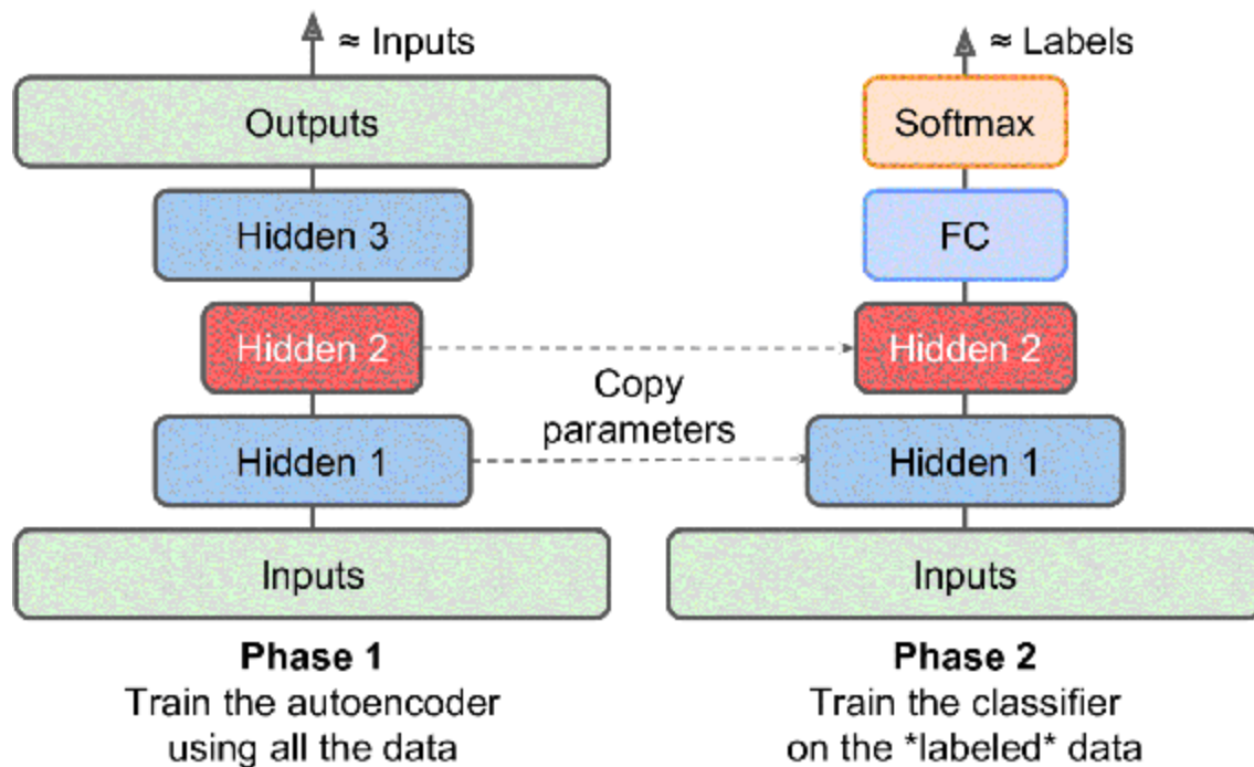
Figure 15-8. Unsupervised pretraining using autoencoders
