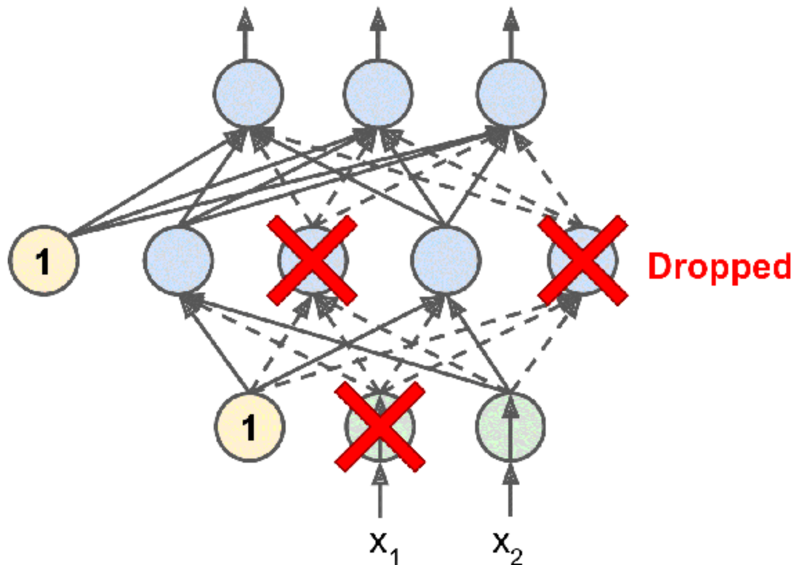
Figure 11-9. Dropout regularization
