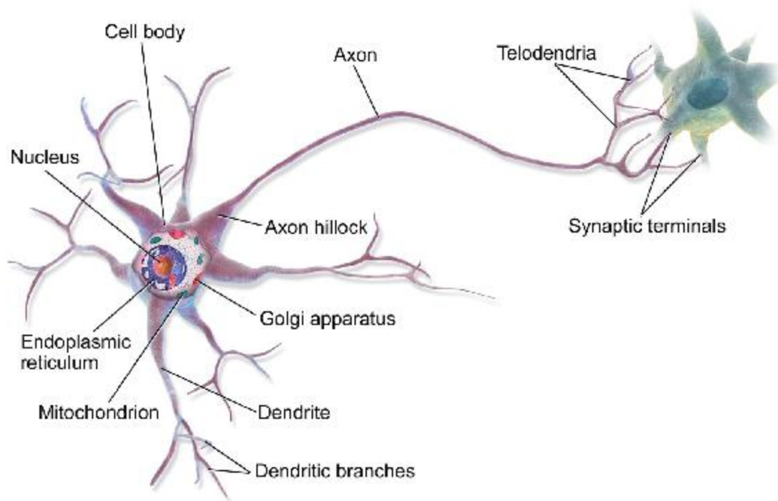
Figure 10-1. Biological neuron 3
