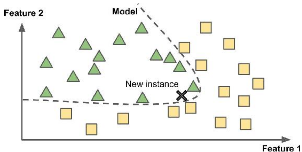
Figure 1-16. Model-based learning
