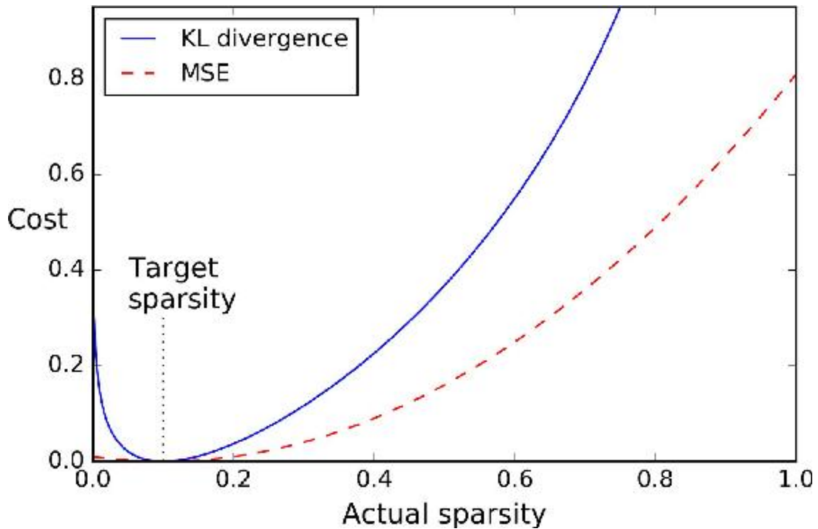
Figure 15-10. Sparsity loss
