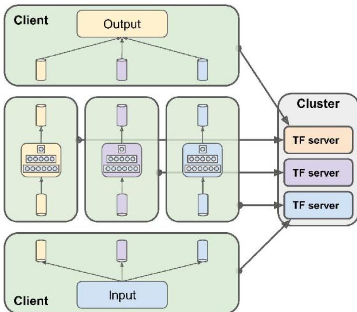
Figure 12-13. Between-graph replication
