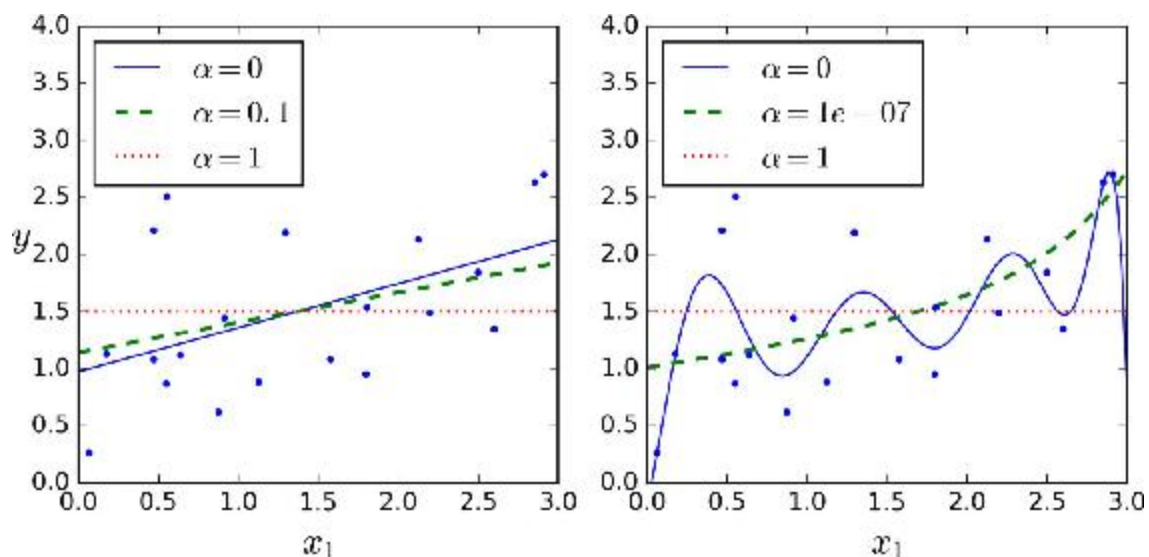
Figure 4-18. Lasso Regression
