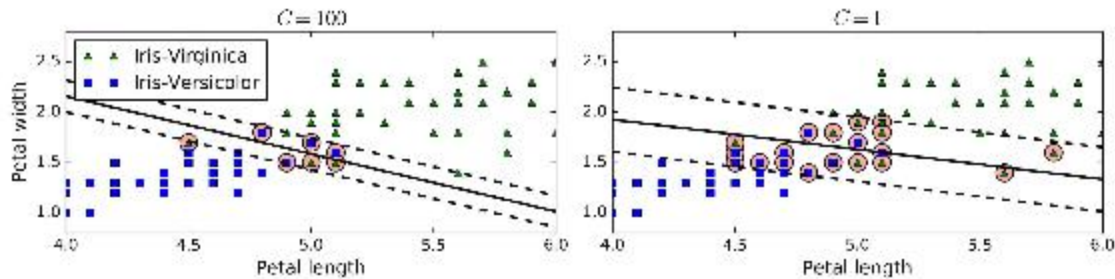
Figure 5-4. Fewer margin violations versus large margin
