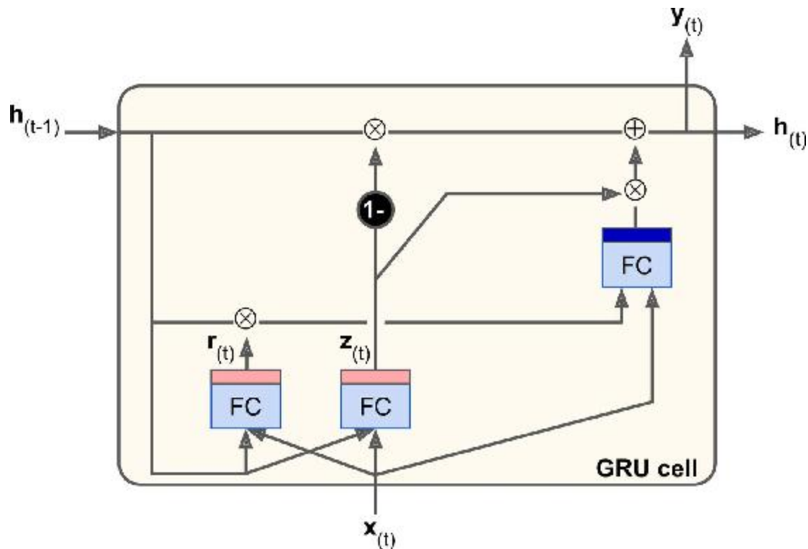
Figure 14-14. GRU cell
