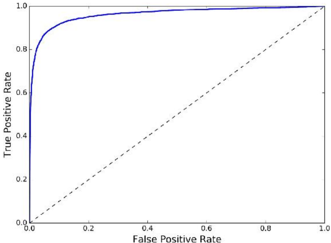
Figure 3-6. ROC curve
