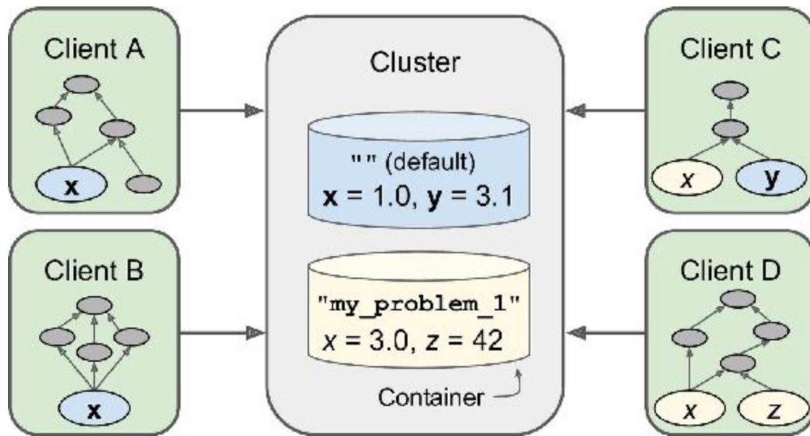
Figure 12-7. Resource containers
