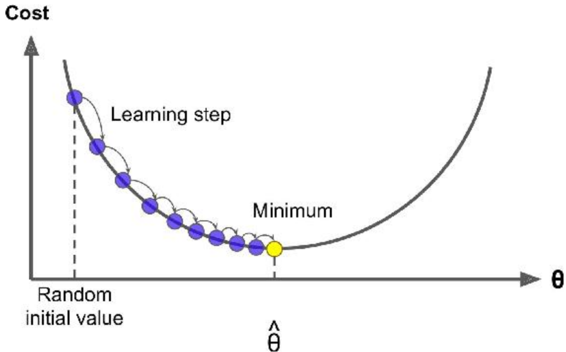
Figure 4-3. Gradient Descent
