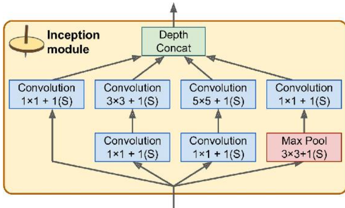
Figure 13-10. Inception module
