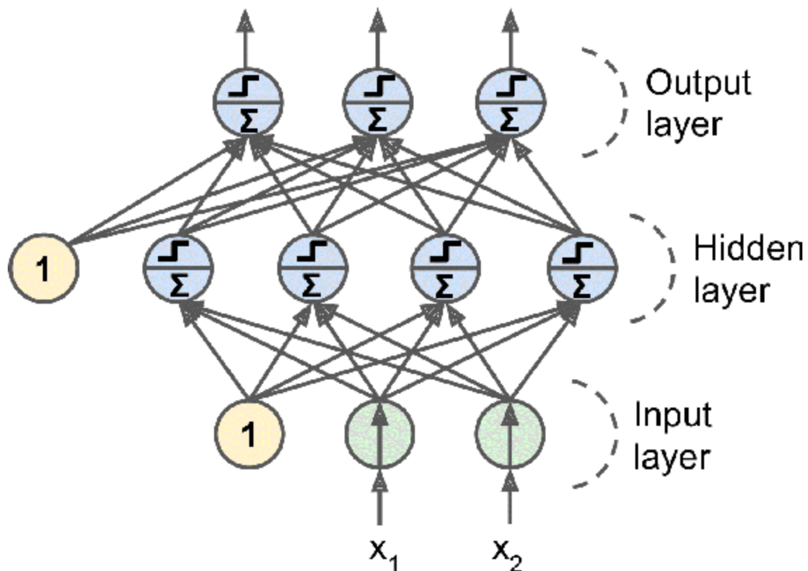
Figure 10-7. Multi-Layer Perceptron
