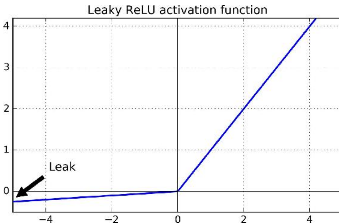
Figure 11-2. Leaky ReLU
