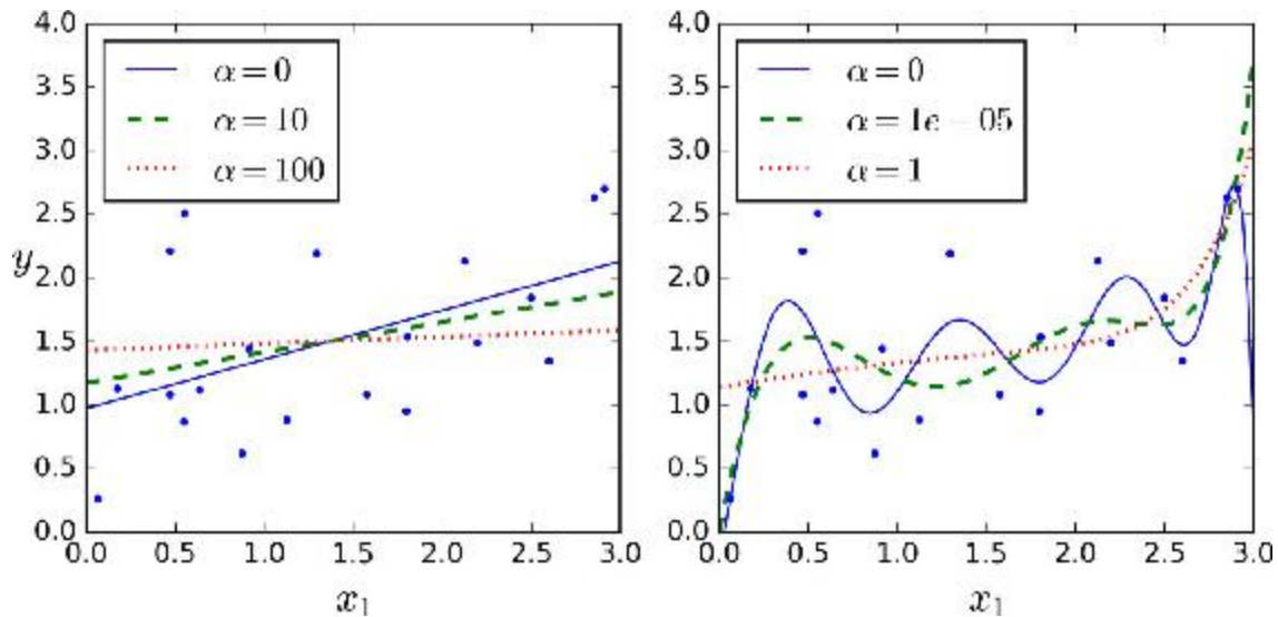
Figure 4-17. Ridge Regression
