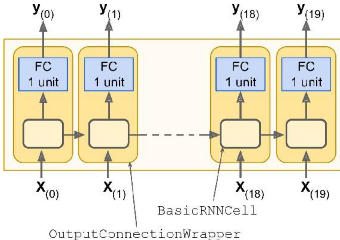
Figure 14-8. RNN cells using output projections
