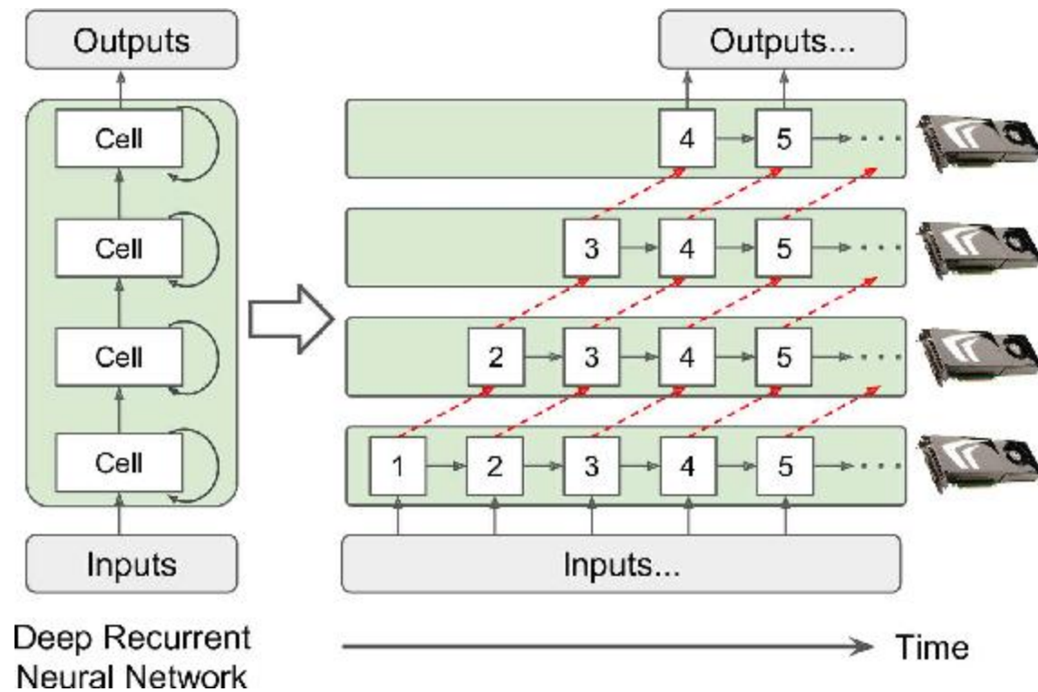
Figure 12-16. Splitting a deep recurrent neural network
