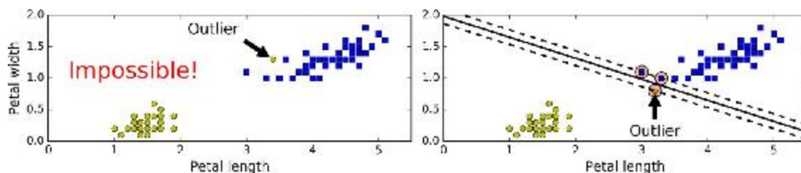
Figure 5-3. Hard margin sensitivity to outliers
