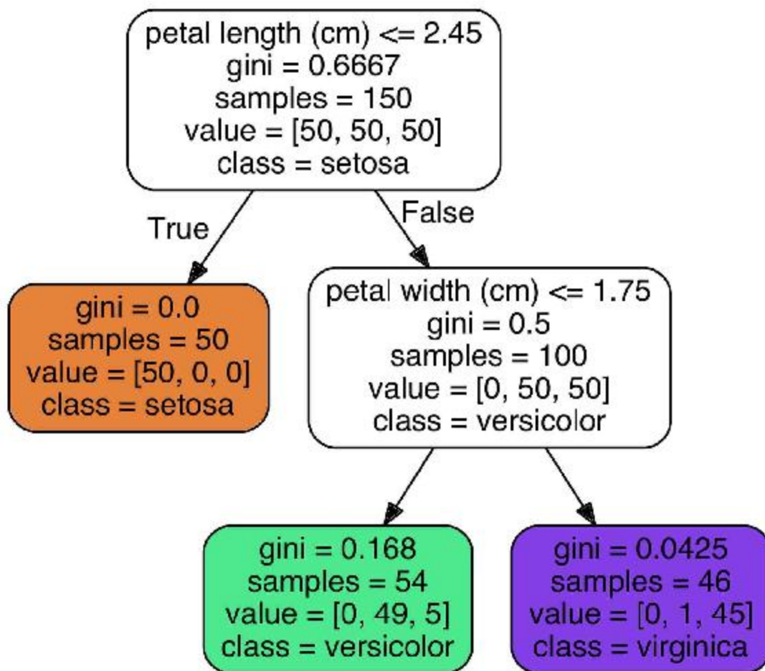
Figure 6-1. Iris Decision Tree
