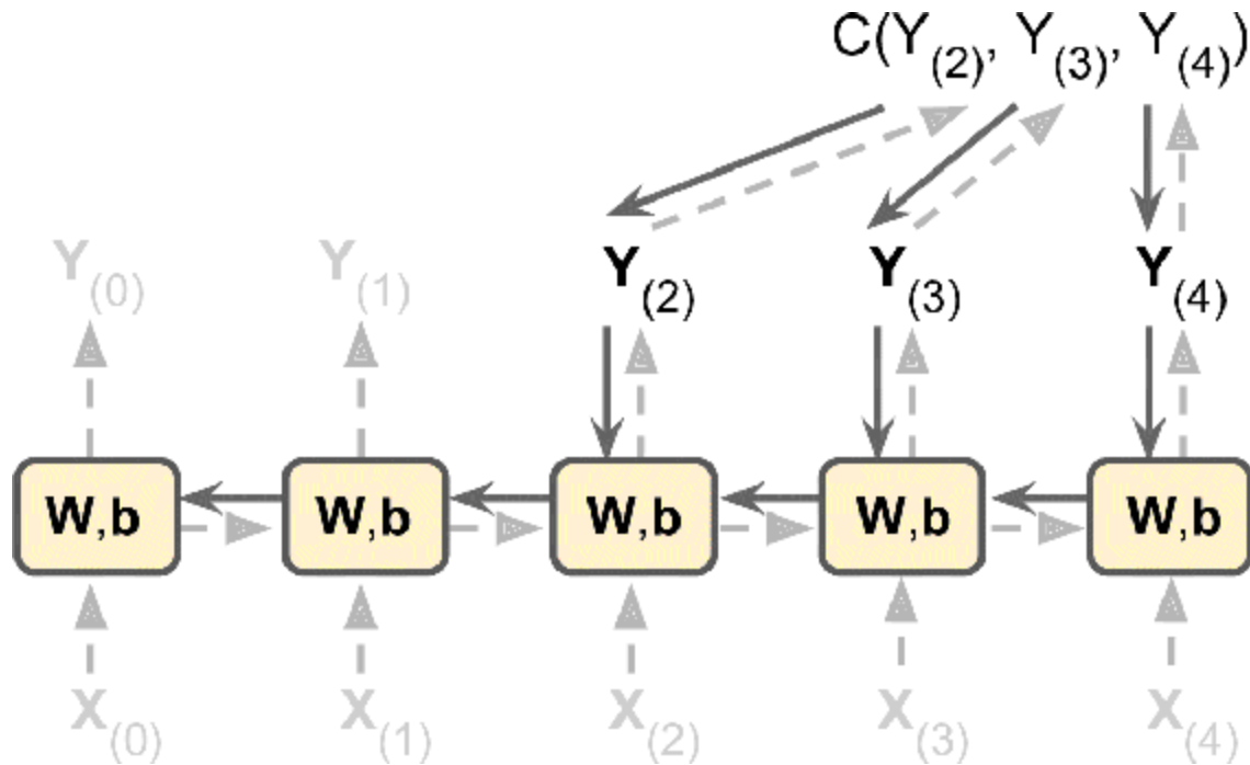
Figure 14-5. Backpropagation through time
