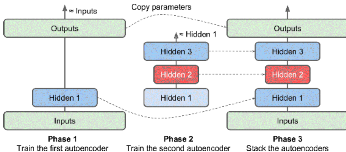
Figure 15-4. Training one autoencoder at a time
