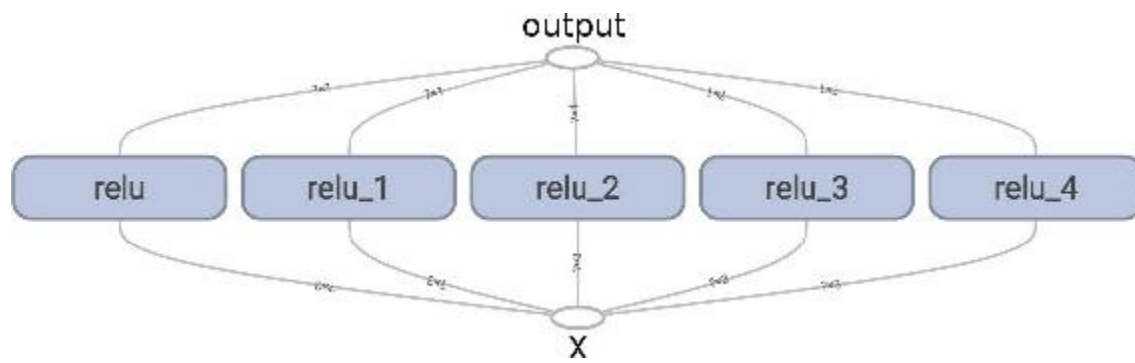
Figure 9-7. A clearer graph using name-scoped units
