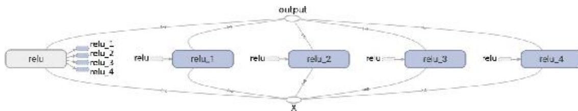
Figure 9-9. Five ReLUs sharing the threshold variable
