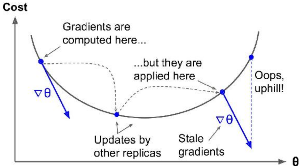
Figure 12-18. Stale gradients when using asynchronous updates
