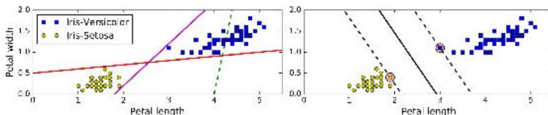
Figure 5-1. Large margin classification
