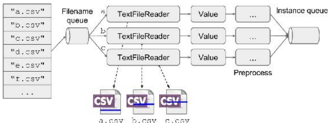
Figure 12-10. Reading simultaneously from multiple files
