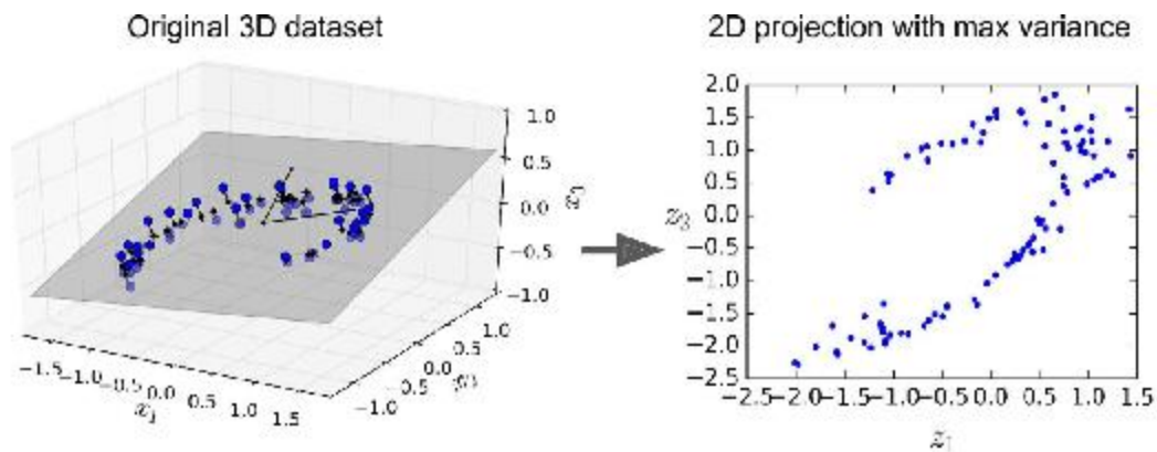
Figure 15-2. PCA performed by an undercomplete linear autoencoder
