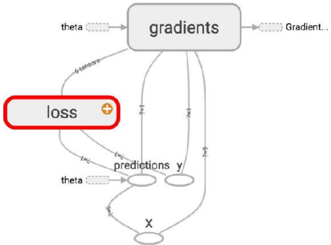
Figure 9-5. A collapsed namespace in TensorBoard
