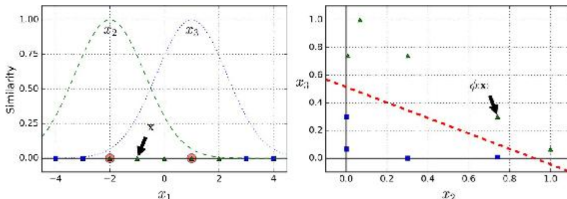
Figure 5-8. Similarity features using the Gaussian RBF
