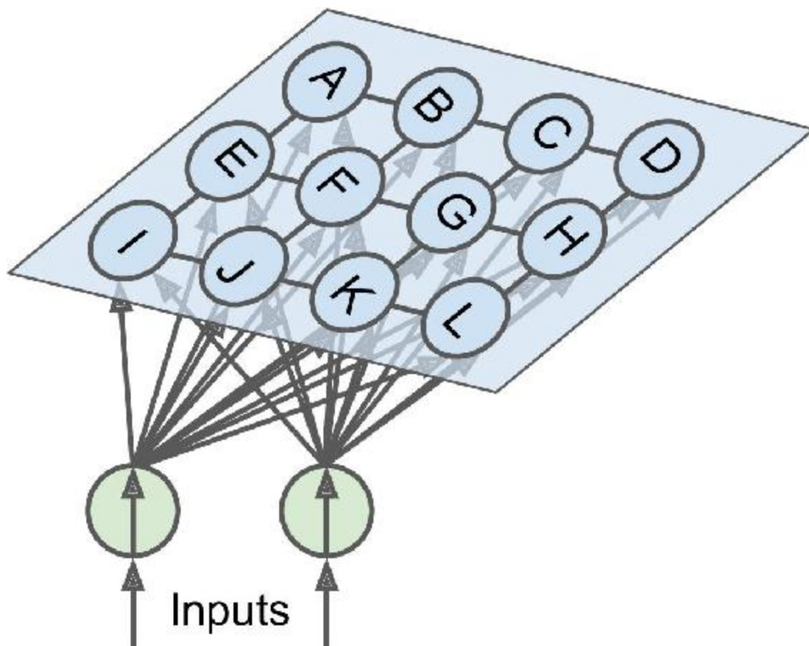
Figure E-5. Self-organizing maps
