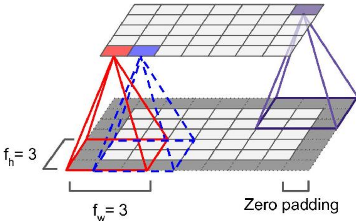
Figure 13-3. Connections between layers and zero padding
