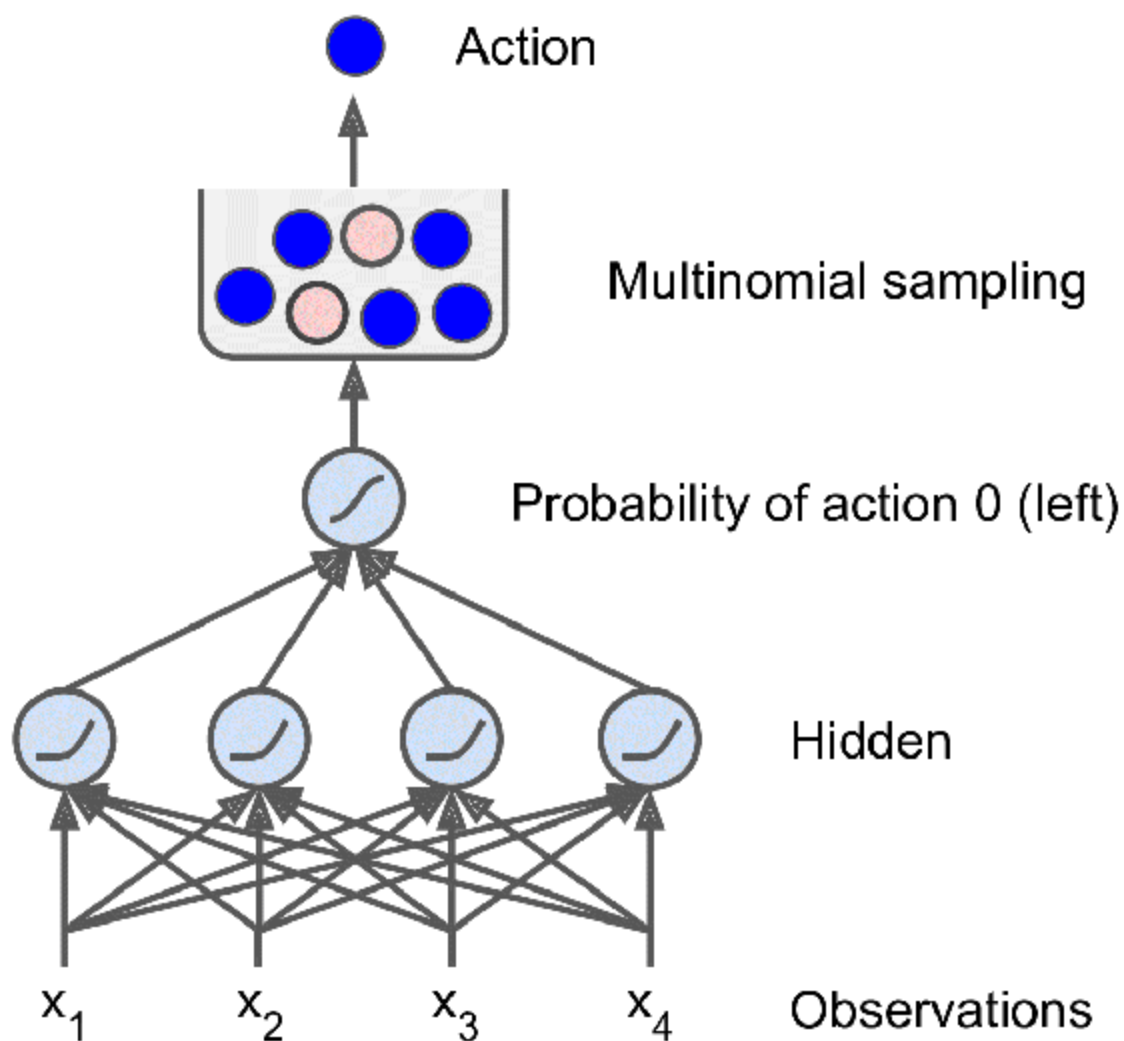
Figure 16-5. Neural network policy
