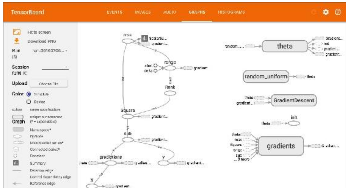
Figure 9-4. Visualizing the graph using TensorBoard
