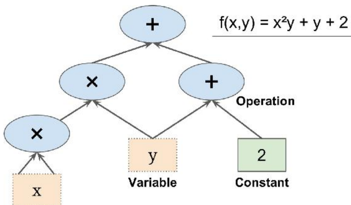
Figure 9-1. A simple computation graph
