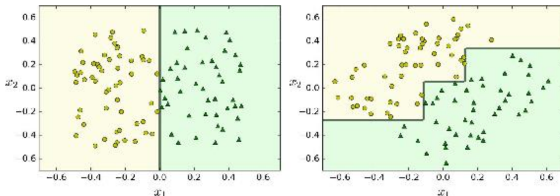
Figure 6-7. Sensitivity to training set rotation
