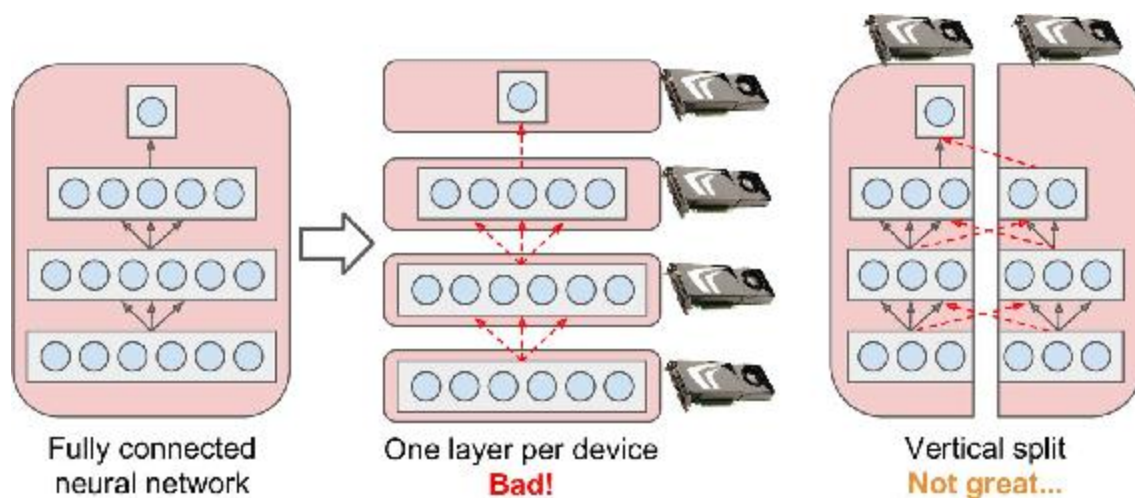
Figure 12-14. Splitting a fully connected neural network
