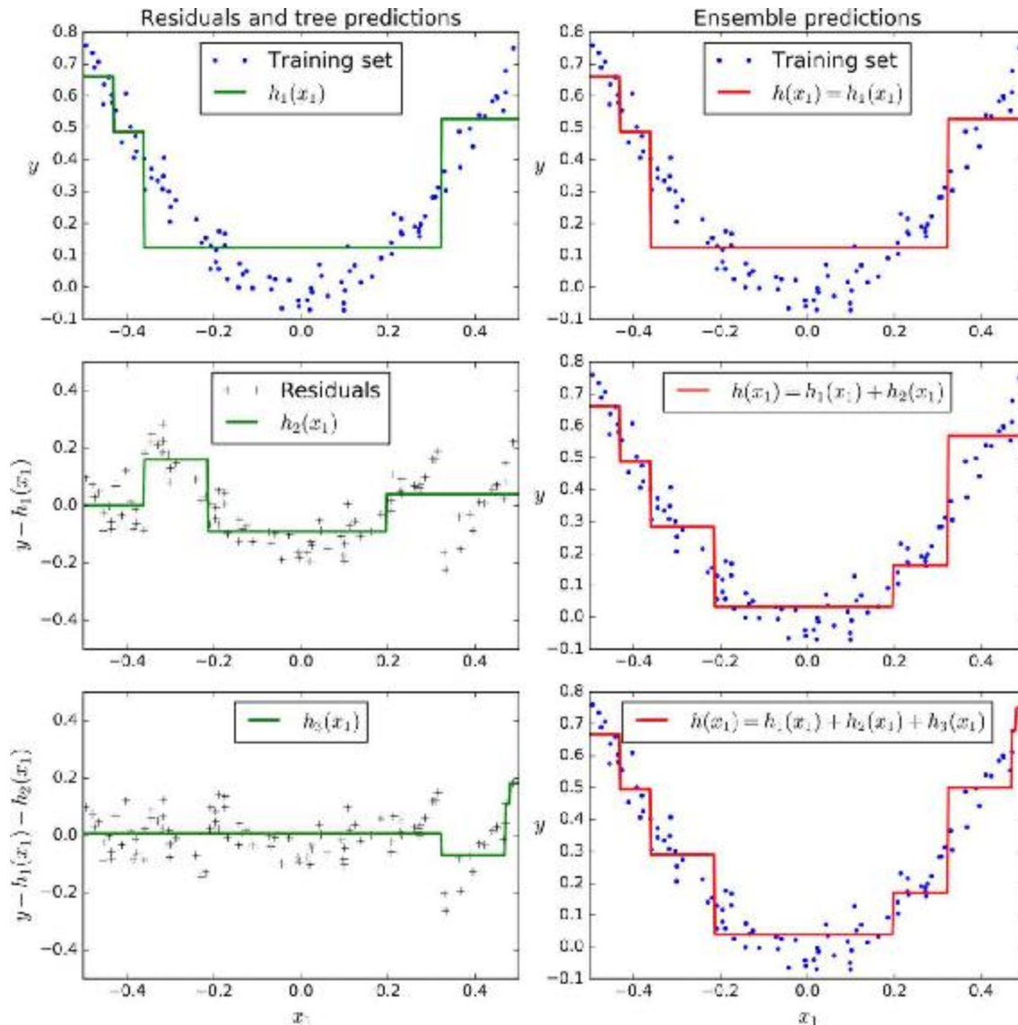
Figure 7-9. Gradient Boosting
