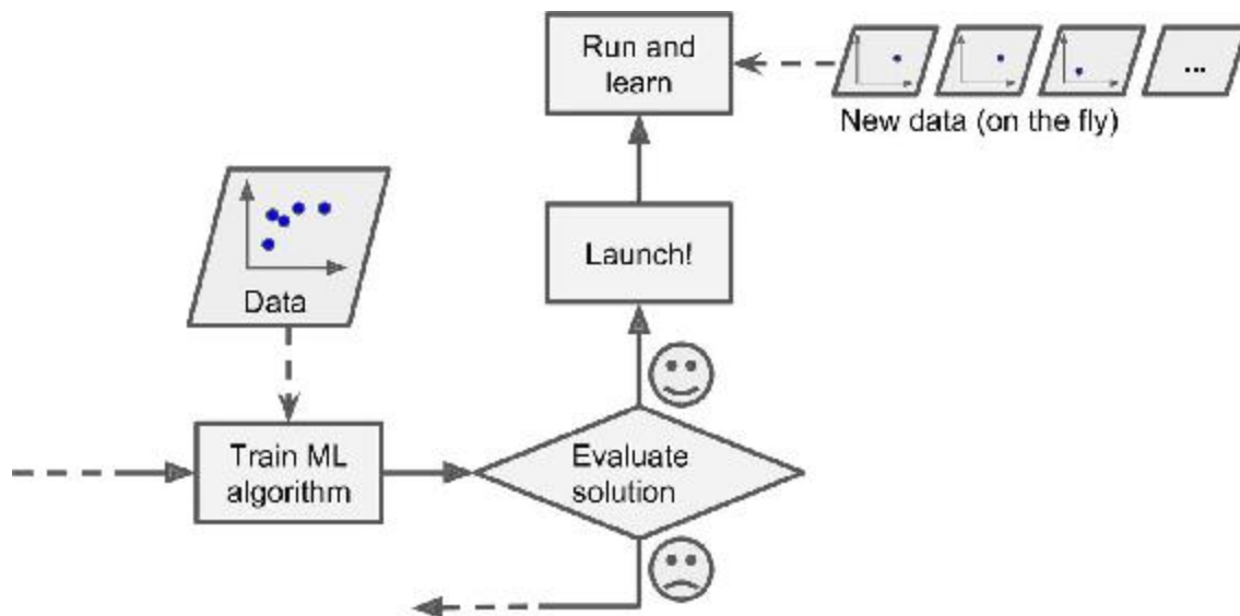
Figure 1-13. Online learning
