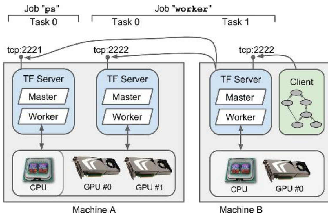
Figure 12-6. TensorFlow cluster
