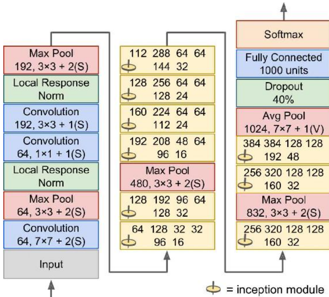
Figure 13-11. GoogLeNet architecture
