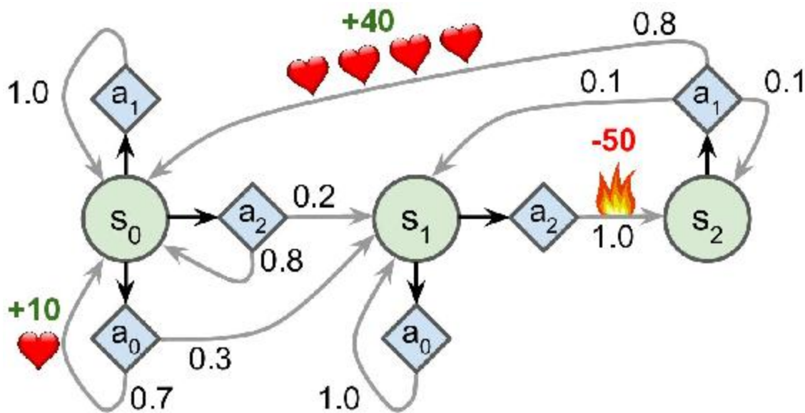
Figure 16-8. Example of a Markov decision process
