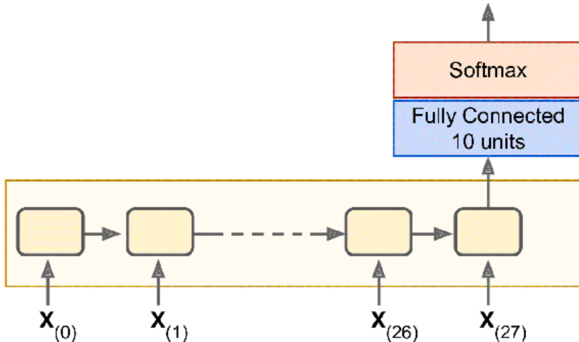
Figure 14-6. Sequence classifier
