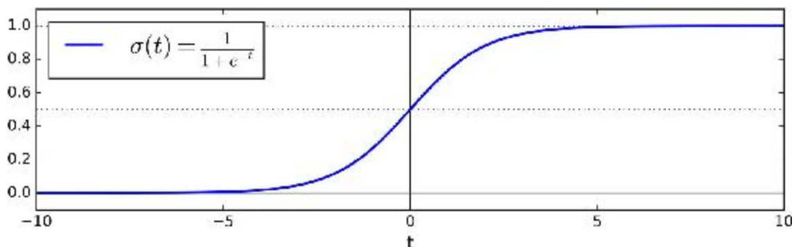
Figure 4-21. Logistic function
