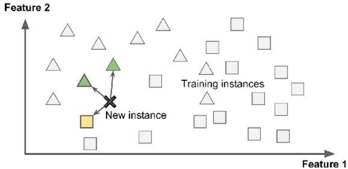
Figure 1-15. Instance-based learning
