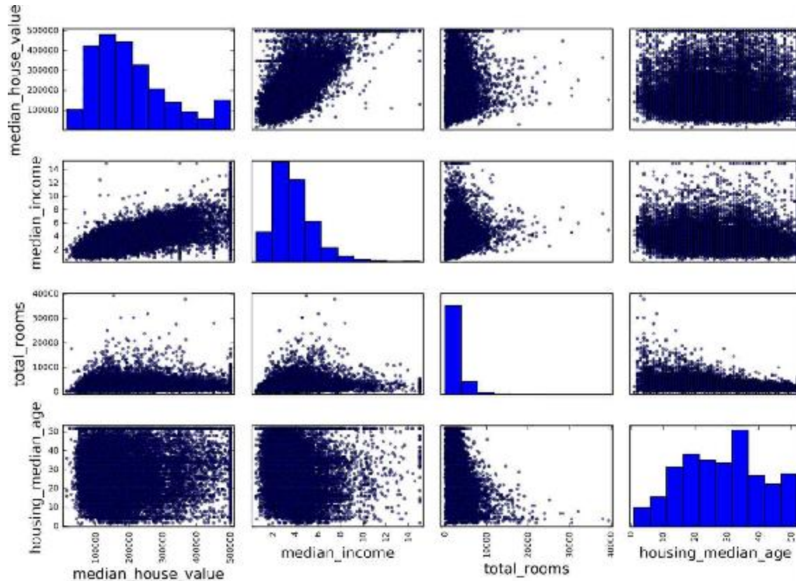
Figure 2-15. Scatter matrix
