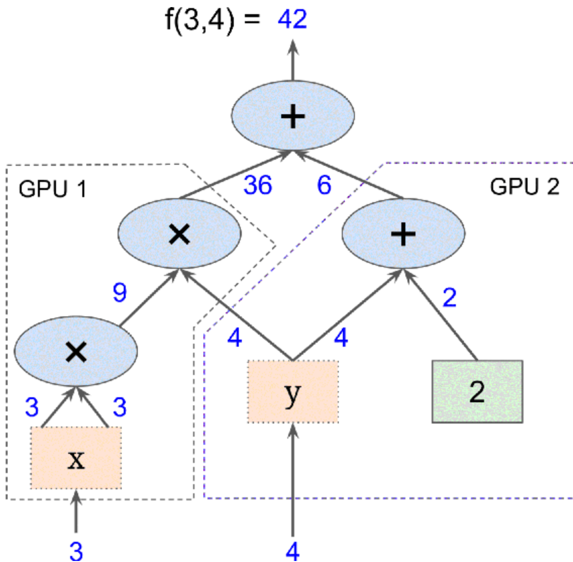
Figure 9-2. Parallel computation on multiple CPUs/GPUs/servers
