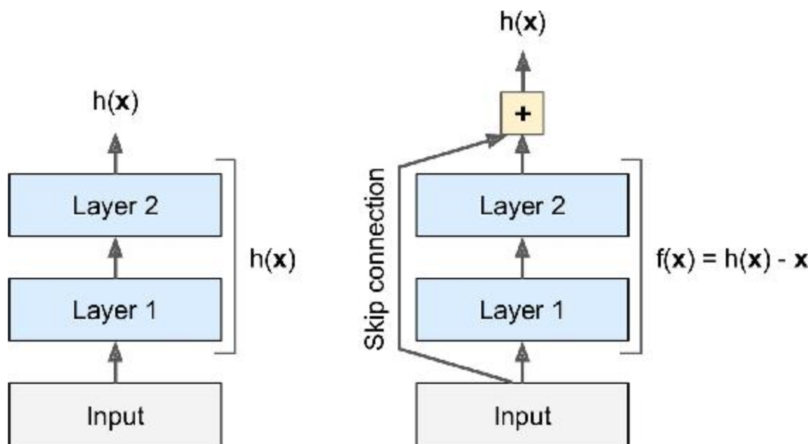
Figure 13-12. Residual learning
