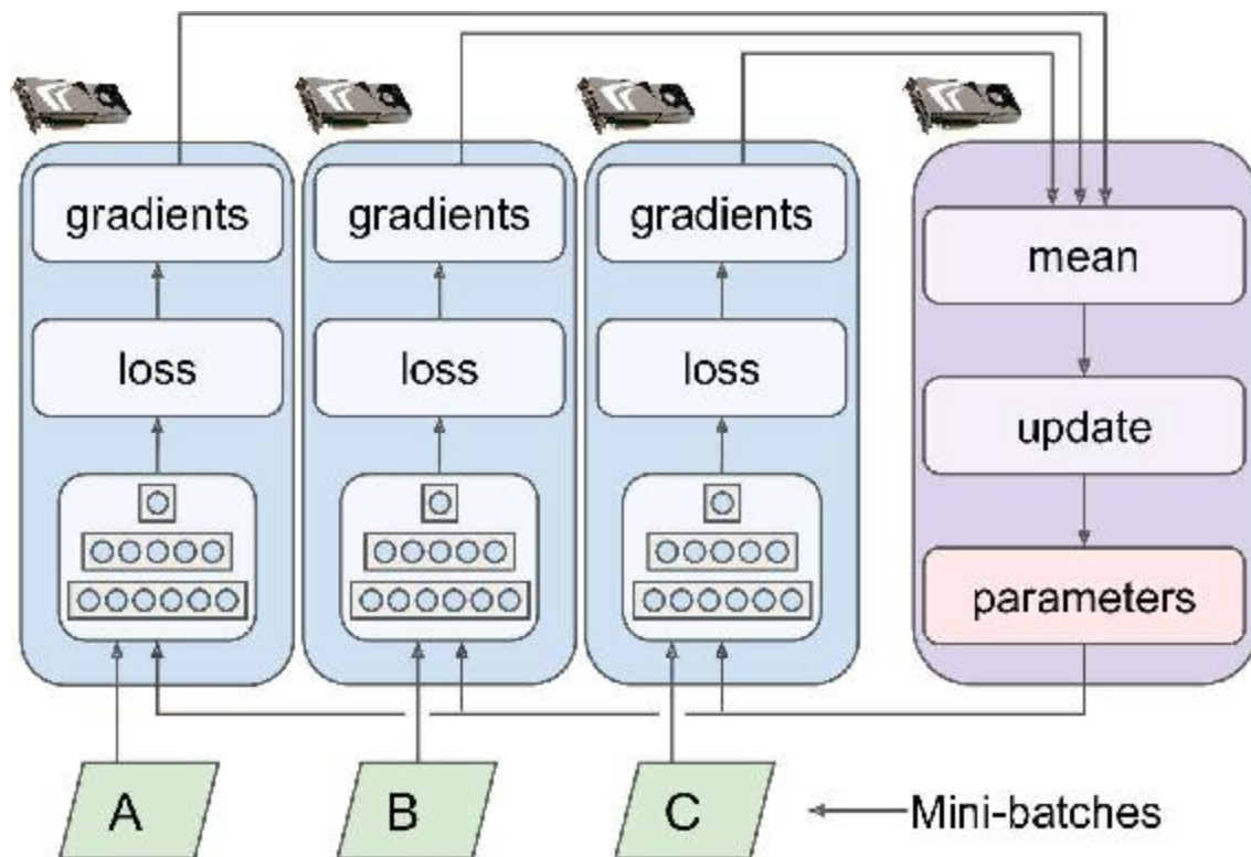
Figure 12-17. Data parallelism
