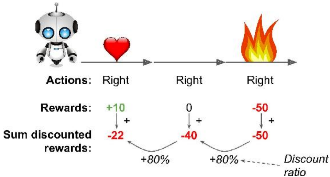
Figure 16-6. Discounted rewards
