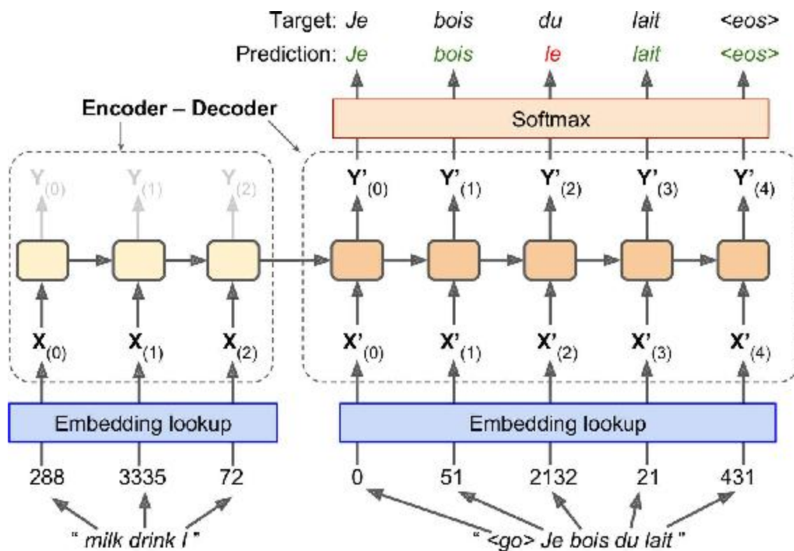
Figure 14-15. A simple machine translation model
