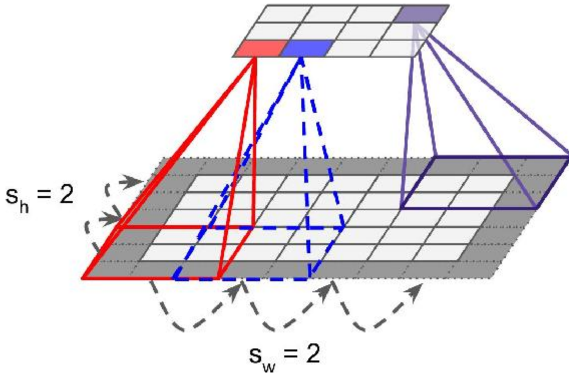
Figure 13-4. Reducing dimensionality using a stride
