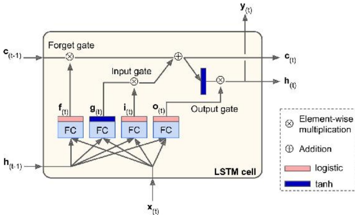
Figure 14-13. LSTM cell
