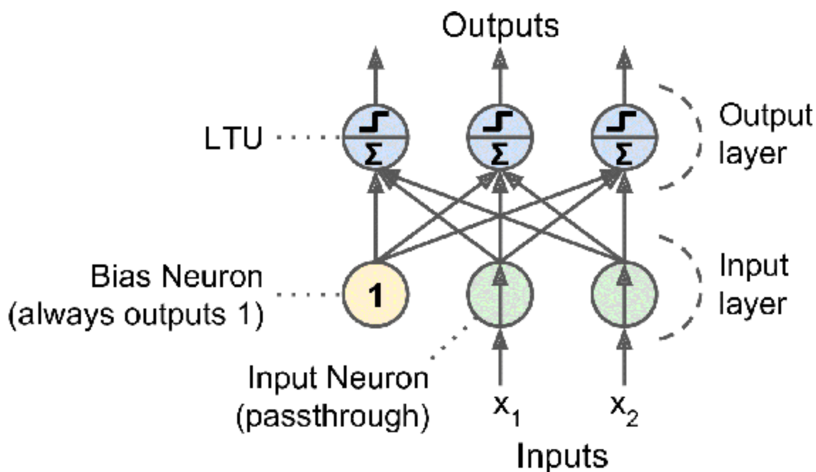
Figure 10-5. Perceptron diagram
