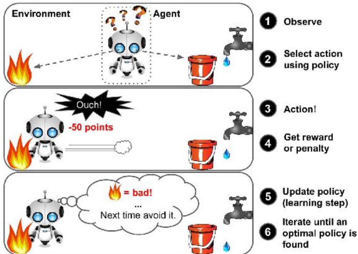
Figure 1-12. Reinforcement Learning
