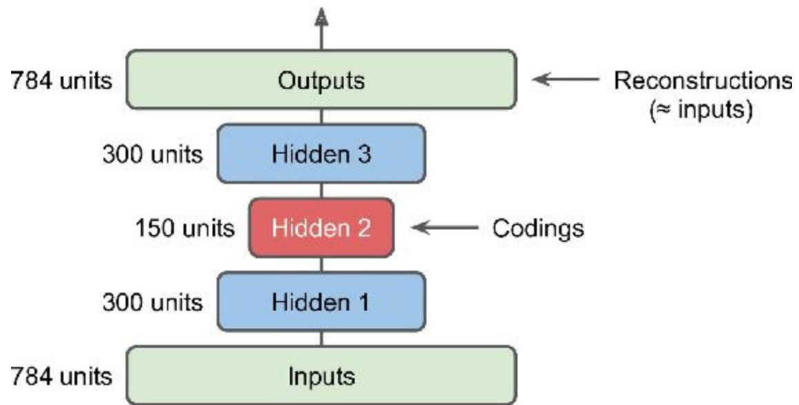
Figure 15-3. Stacked autoencoder
