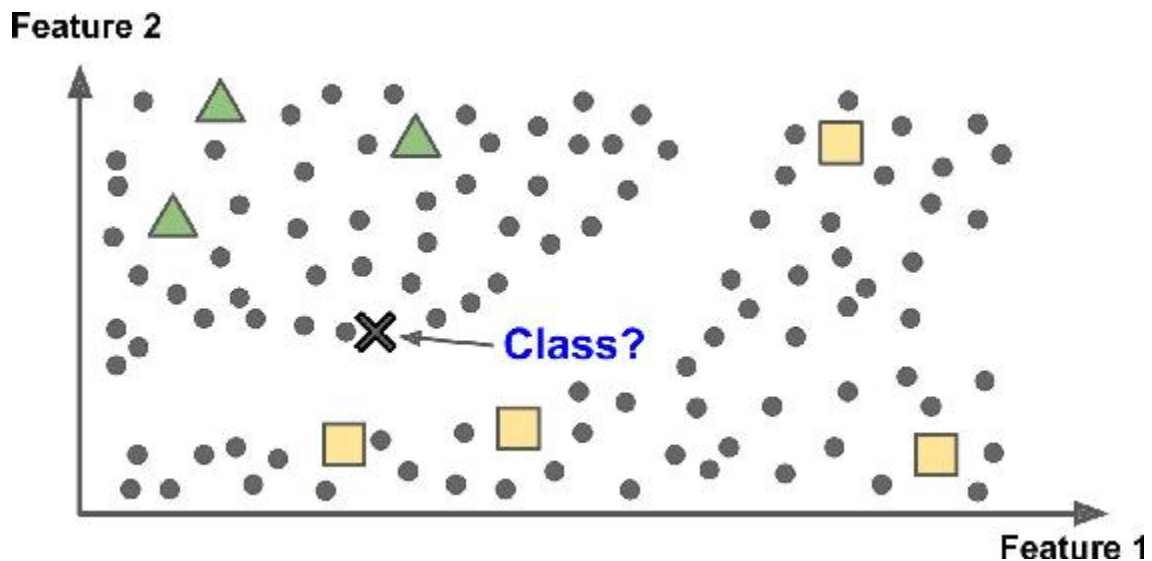
Figure 1-11. Semisupervised learning
