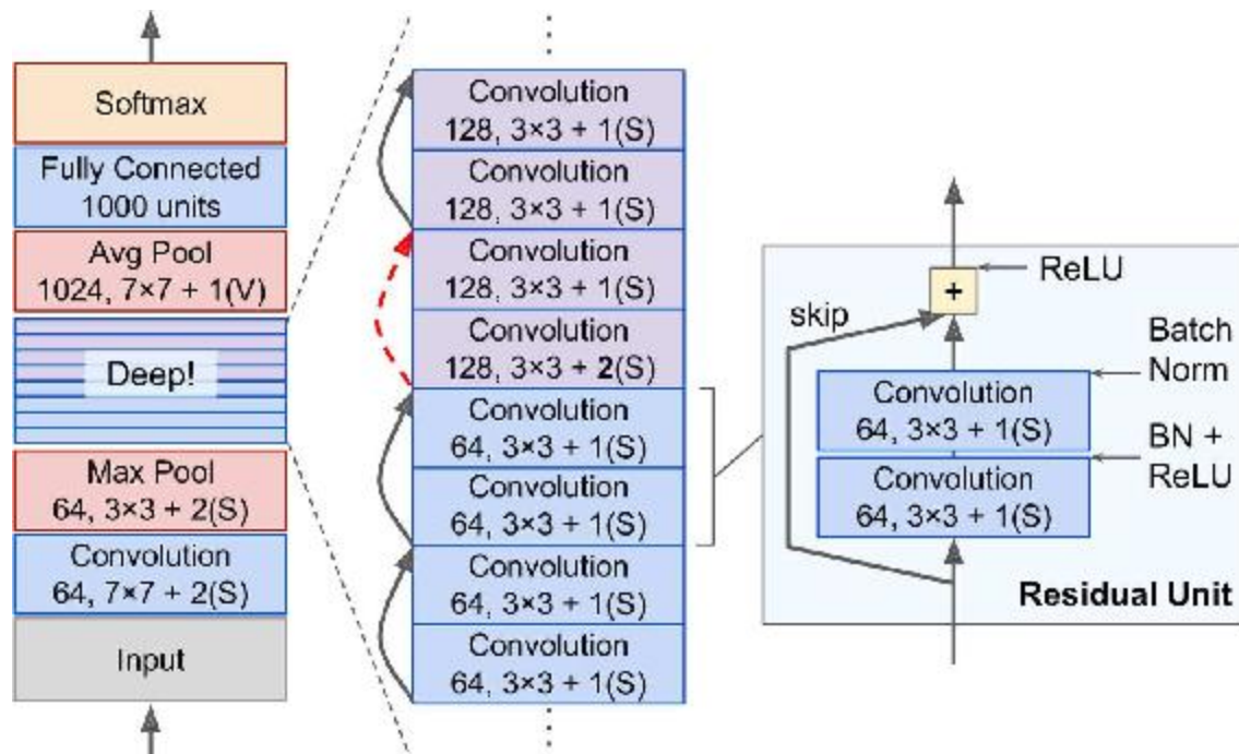
Figure 13-14. ResNet architecture
