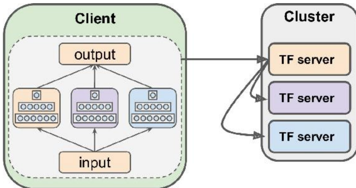
Figure 12-12. In-graph replication
