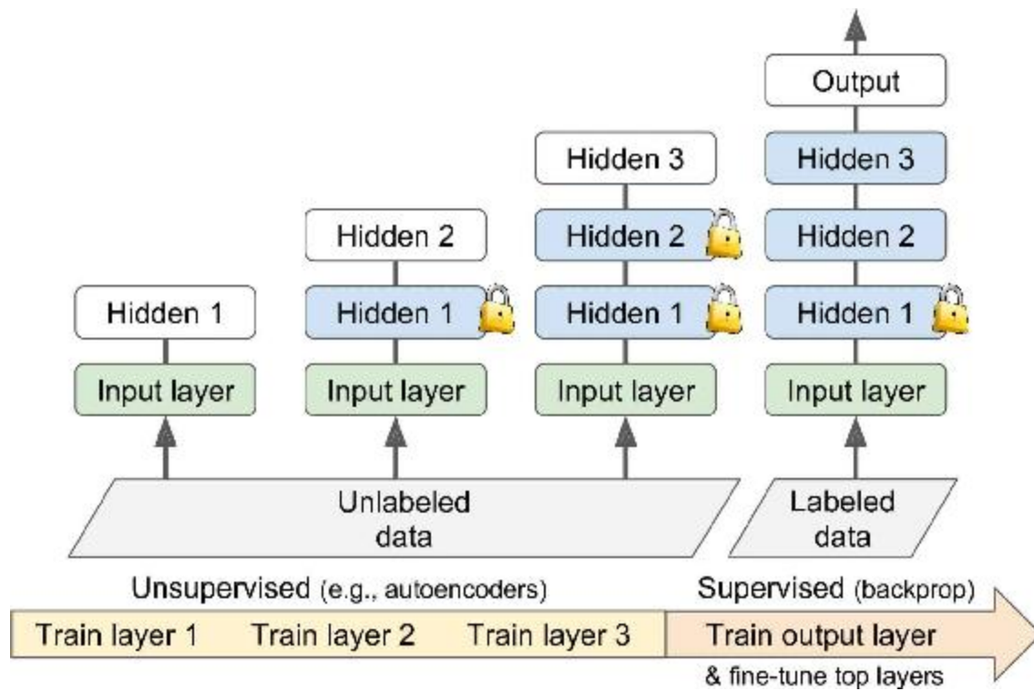
Figure 11-5. Unsupervised pretraining
