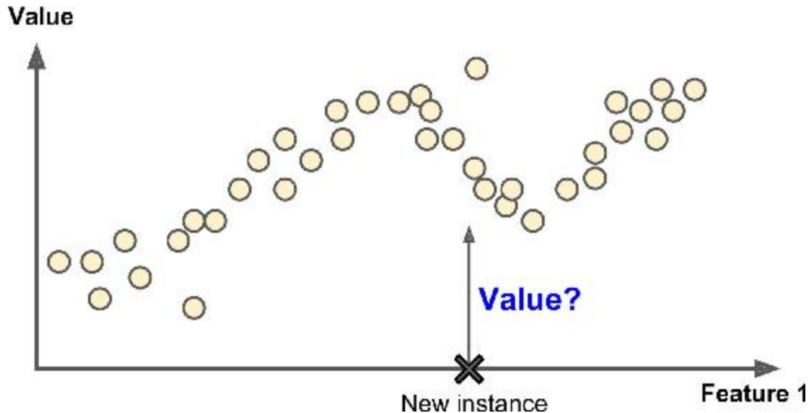
Figure 1-6. Regression
