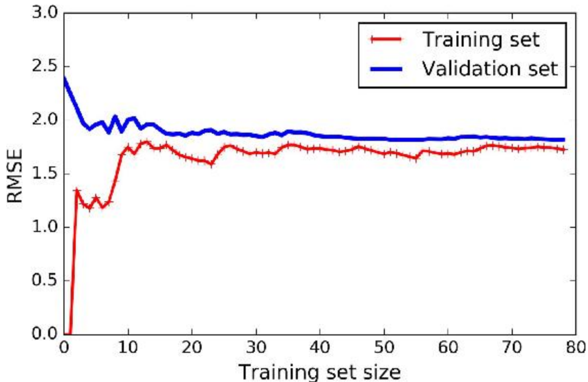
Figure 4-15. Learning curves
