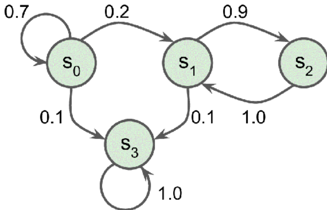
Figure 16-7. Example of a Markov chain
