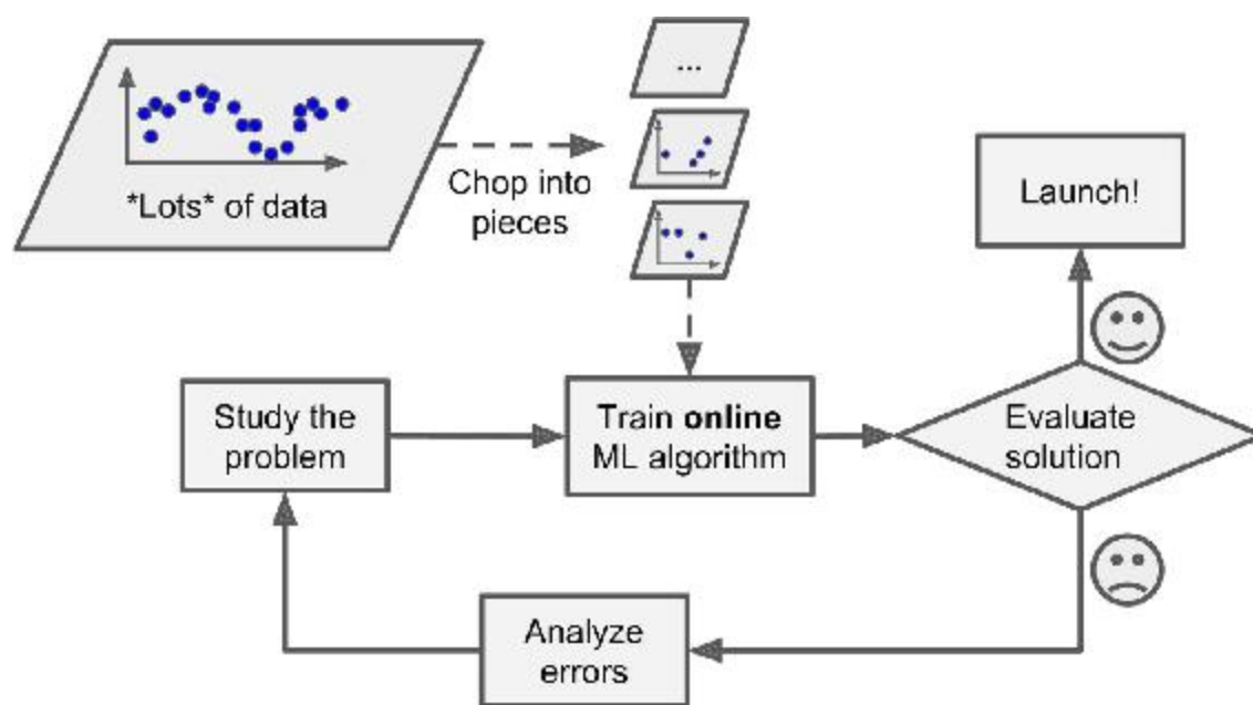
Figure 1-14. Using online learning to handle huge datasets
