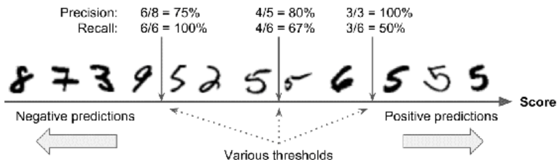
Figure 3-3. Decision threshold and precision/recall tradeoff
