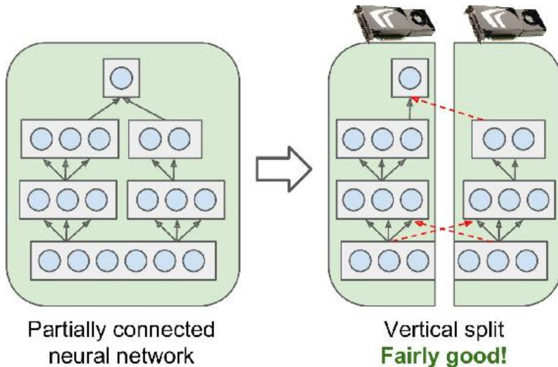
Figure 12-15. Splitting a partially connected neural network
