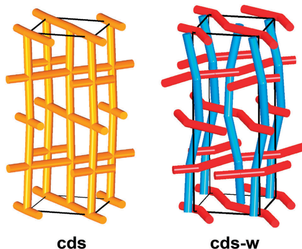
Fig. 20 A weaving derived from the cds net shown on left.
