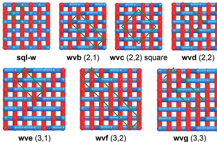
Fig. 8 The simplest biaxial weavings. All but wvc are twills.
