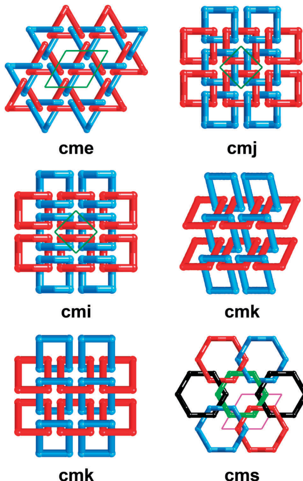
Fig. 12 2-Periodic linked rings with symmetry related link points that form the kgm (3.6.3.6) or sql ( 4^4 ) nets. cmk ('European four-in-one chain mail') shown twice is the only one with an embedding with planar rings.
