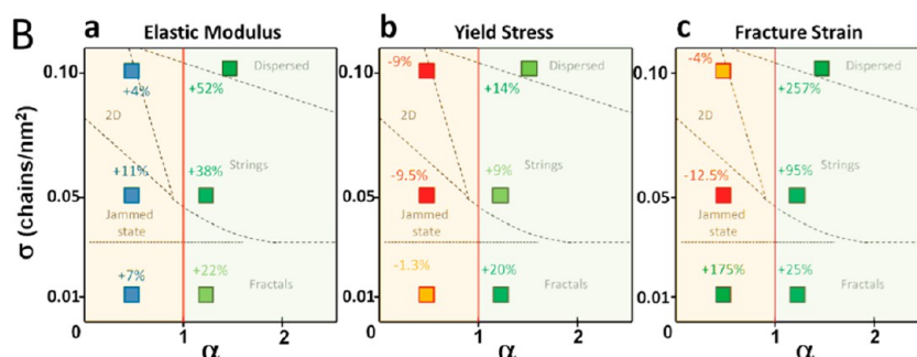
Figure 11. Reinforcement percentage of the (a) elastic modulus, (b) yield stress, and (c) failure strain relative to the pure polymer depending on grafting density \sigma and grafted/matrix chain lengths ratio \alpha . The loading of the silica core was 5 mass % in all the samples, and the morphologies of NP in these thin films are those reported in ref 56. Reproduced from ref 199.
