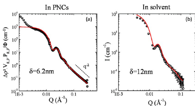
Figure 3. Grafted chain thickness \delta in (a) PNCs and in (b) solvent as determined by small-angle neutron scattering (SANS). Using an appropriate contrast variation, one can match the silica scattering to the matrix polymer and thus only measure the signal of the grafted corona. The continuous lines are the best fits using a Gaussian chain model (a) and a “core/shell” model (b). Adapted from ref 147.
