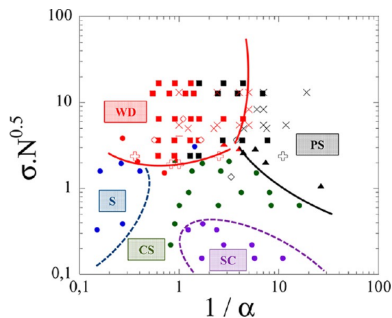
Figure 4. A composite morphology diagram created from all of the available data in the literature: \sigma\sqrt{N} as a function of 1/\alpha with \alpha = N/P . The points, adapted from the literature, are color coded so that a red point corresponds to well dispersed particles (WD); black to phase separated samples (PS); blue to strings (S); green to connected sheets (CS) and purple to small clusters (SC). The color-coded lines represent a first-order cut at classifying the data into well defined regions in the plot where different morphologies occur. This classification is not perfect – for example, there are black squares in a red region. ( \square ) is for 18 nm PS-g-SiO 2 NP from ref 29, ( \times ) for 10 nm PEO-g-SiO 2 NP from ref 44, ( \blacklozenge ) for 17 nm PS-g-SiO 2 NP from ref 160, ( \bullet ) for 14 nm PS-g-SiO 2 NP from ref 46, ( \triangle ) for 28 nm PS-g-SiO 2 NP from ref 154, ( - ) for 12 nm PBA-g-SiO 2 NP from ref 207, and ( + ) for 8 nm PS-g- \gamma -Fe 2 O 3 NP from ref 220.
