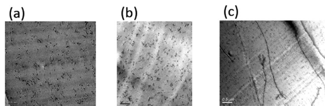
Figure 6. Time evolution of the bulk structures formed by 14 nm diameter silica NP grafted with PS chains ( 106\text{K} , 0.05 chains/ \text{nm}^2 ) in a PS matrix ( 231\text{K} ): (a) as cast, (b) annealed for 3 days, and (c) annealed for 5 days at 150 °C. The samples were annealed for up to 28 days, and the structures continue to grow.
