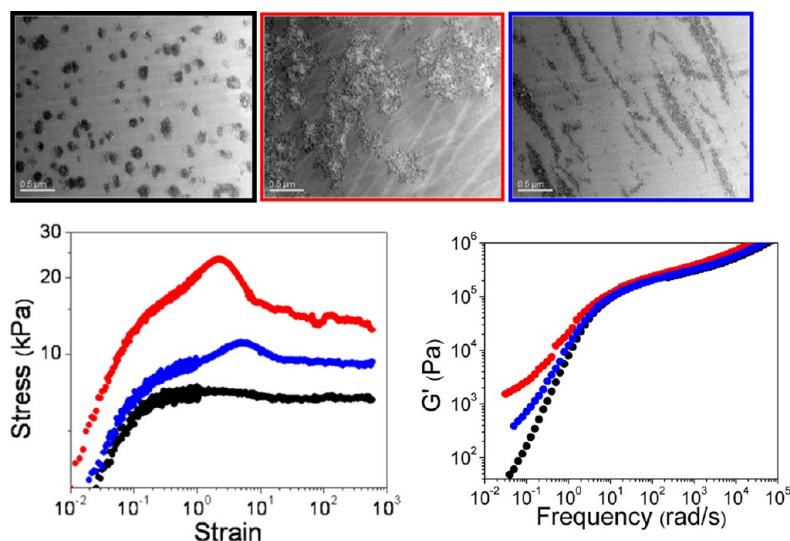
Figure 9. (A) TEM images showing nanoparticle dispersion states. All three samples have a 142 kg/mol matrix. Left: agglomerated, 25 kg/mol graft, 0.01 chains/nm 2 (black). Center: a particle network, 17 kg/mol graft, 0.05 chains/nm 2 (red). Right: sheets of particles, 24 kg/mol graft, 0.1 chains/nm 2 (blue). (B) Steady shear data at 180 °C at a shear rate of 0.2/s. (C) Storage modulus data for the same three nanocomposites, also taken at 180 °C. Reproduced from ref 57.
