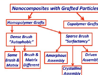
Figure 1. Broad area covered by review. Discussion is primarily on the left side of this diagram, in the case of “homopolymer” brushes.
