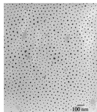
Figure 8. TEM micrograph of 14 nm silica nanoparticles grafted with a 80K poly( n -butyl acrylate). The sample was drop-cast on a TEM grid and then imaged. Adapted from ref 155.
