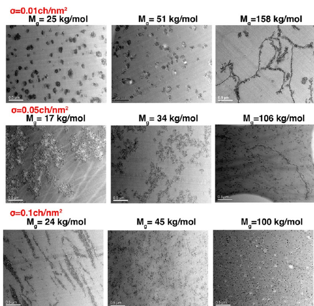
Figure 5. TEM determined temporal structuring. In all cases 5 mass % silica grafted with a variety of graft molecular weights, M_g , of a polystyrene brush with varying grafting densities, \sigma , is mixed with polystyrene matrices of M = 142 kg/mol and annealed at 150 °C for 5 days. The scale bars are 0.5 \mu\text{m} . Adapted from reference 46.
