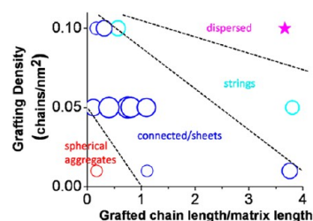
Figure 10. In a “morphology” diagram we plot symbols whose size scale with the degree of reinforcement as characterized by the ratio (stress overshoot maximum value)/(plateau value). Other measures give qualitatively similar results. Only the well-dispersed sample yielded no stress maximum. Reproduced from ref 57.
