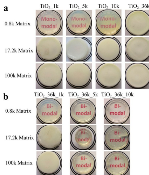
Figure 12. Visualization of nanocomposites formed by TiO 2 grafted with PDMS in a PDMS matrix. Reproduced from ref 120.
