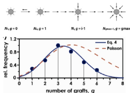
Figure 2. (top) Schematic representation of the surface functionalization reaction. The total number of reactive sites per particle is g_{\max} . The coupling of functional ligands is assumed to proceed by a sequence of irreversible coupling reactions with equal and constant rate. (bottom) Distribution of the number of grafting sites per particle. The dotted line is a Poisson distribution, while the solid line is derived from a population balance model. Adapted from ref 124.
