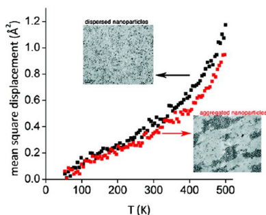
Figure 7. Mean-square displacement \langle u^2 \rangle obtained by QENS for well-dispersed (black symbol) and aggregated (red symbol) NP states. Reproduced from ref 184.
