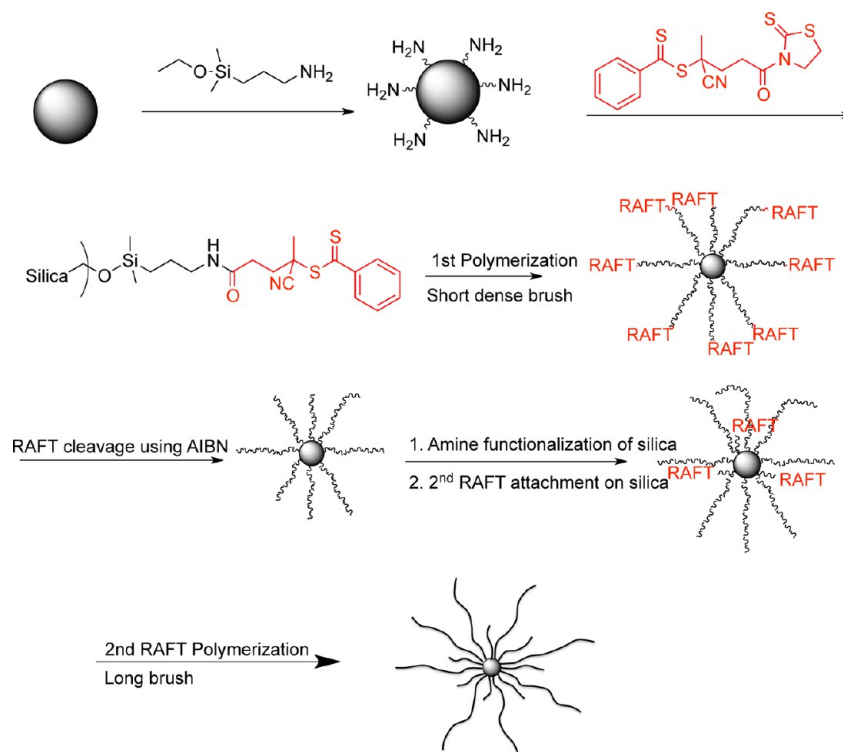
Scheme 1. Synthesis of Bimodal Brush Particles Using Sequential RAFT Polymerization
