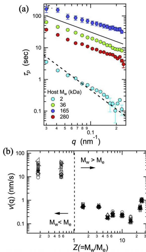
Fig. 17. (a) Nanoparticle relaxation time as a function of q for PEG functionalized SiO 2 in PMMA of varying molecular weight. Solid line denotes superdiffusion ( q^{-1} ) and dashed line denotes Brownian diffusion ( q^{-2} ). (b) NP velocity extracted as the slope of (a) as a function of entanglements per chain [159]. Copyright 2016. Adapted with permission from the American Chemical Society.
