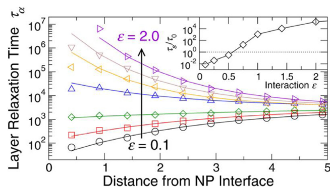
Fig. 7. Segmental relaxation time for \epsilon = 0.1, 0.25, 0.5, 0.75, 1.0, 1.4 , and 2.0 as a function of distance from the NP surface. Inset shows surface segmental relaxation time (normalized to that of bulk) as a function of interaction strength [119]. Copyright 2016.
