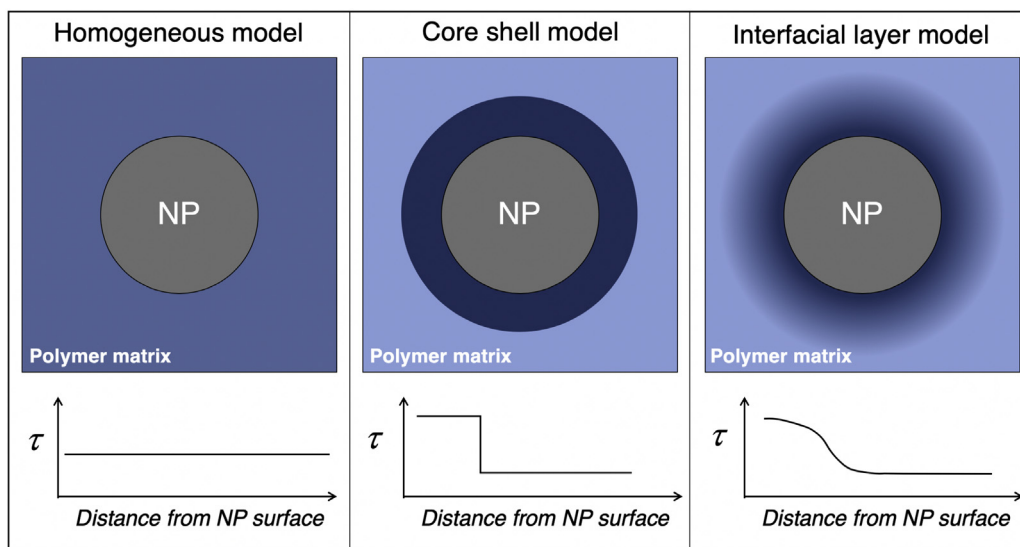
Fig. 3. Schematic showing polymer segmental dynamics as a function of distance from a single NP. The homogeneous model (left) assumes an average relaxation time throughout the polymer matrix. The core-shell model (center) spatially separates the polymer relaxations into a slower population adjacent to the NP and another bulk-like population away from the NP surface. The interfacial layer model (right) assumes a distribution of relaxation times that decreases smoothly from the NP surface into the matrix.
