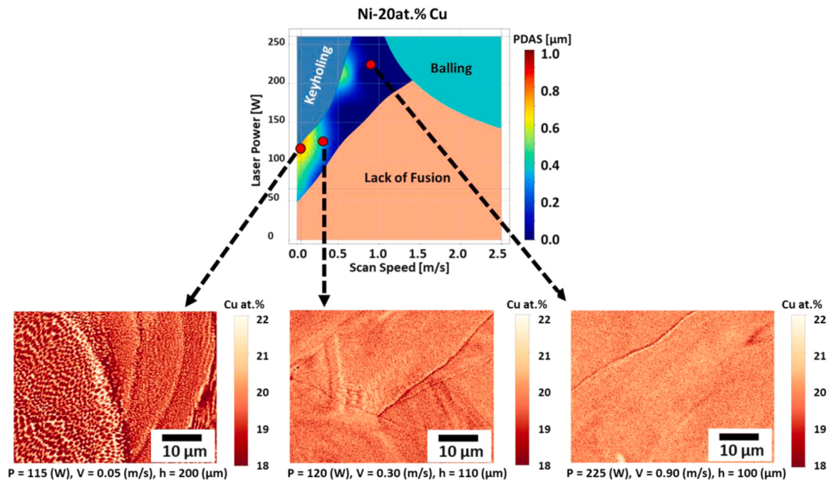
Fig. 12. A combined Porosity-Microstructure processing map for Ni-20 at.% Cu, as well as wavelength dispersive spectroscopy (WDS) composition maps taken from each of the printed cubes listed in Table 2. The cubes were printed at \{P = 115 \text{ W}, v = 0.05 \text{ m/s}, h = 200 \mu\text{m}\} , \{P = 120 \text{ W}, v = 0.30 \text{ m/s}, h = 110 \mu\text{m}\} , and \{P = 225 \text{ W}, v = 0.90 \text{ m/s}, h = 100 \mu\text{m}\} .
