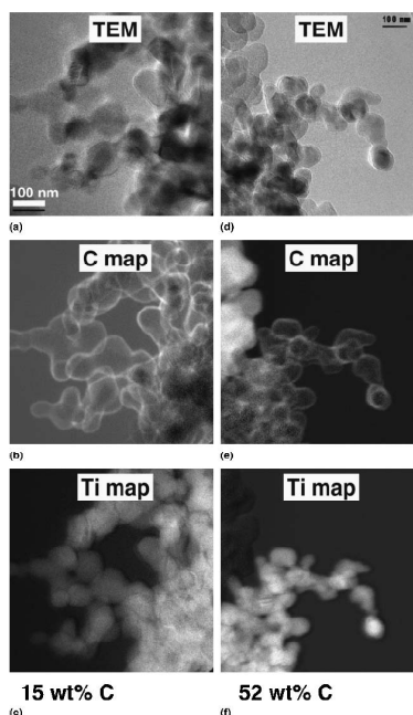
Figure 2.4. Carbon coated titania nanoparticles produced in a diffusion flame by Kammler and Pratsinis (collaborators of Beaucage) [ Carbon-coated titania nanostructured particles: Continuous, one-step flame-synthesis Kammler HK and Pratsinis SE, J. Mater. Res. 18 2670-76 (2003)].
