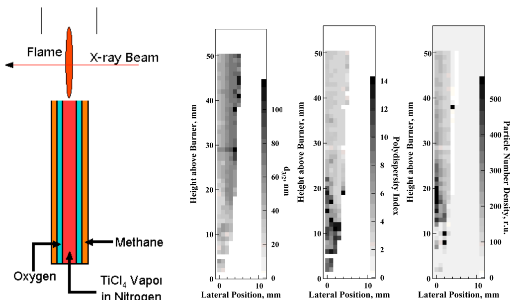
Figure 2.3. Schematic of \text{TiCl}_4 diffusion flame and 2D maps of Sauter mean diameter, particle size polydispersity, and particle number density. The diffusion flame displays a combustion front away from the centerline (lateral position = 0). Higher flame temperatures lead to larger particles with lower polydispersity and lower particle number density.
