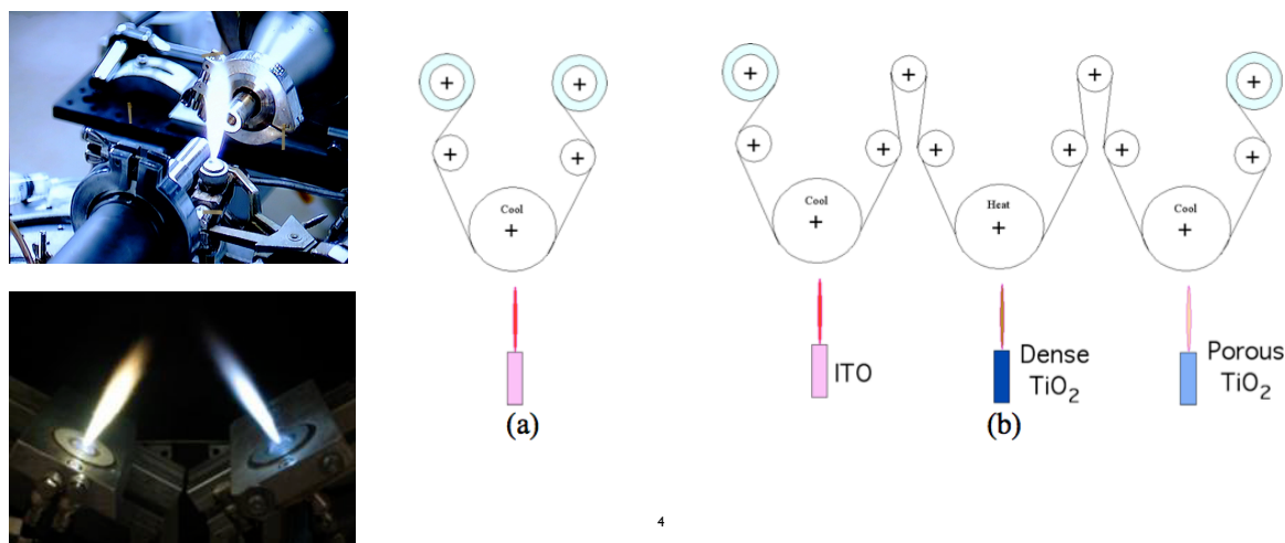
Figure 4.10. Deposition of Nanostructured Coatings using flame pyrolysis: a) single layer coating used for the production of a nanoporous substrate, b) in-line deposition of multiple layers for the production of a Grätzel cell.
