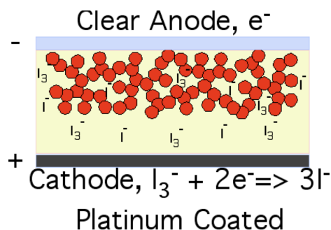
Figure 4.7 Schematic of a Grätzel Cell. Red circles are titania aggregates coated with a dye. The yellow background is an iodide electrolyte gel. Platinum coated cathode is at the bottom and a clear plastic sheet coated with fluorine doped tin oxide anode is at the top.
