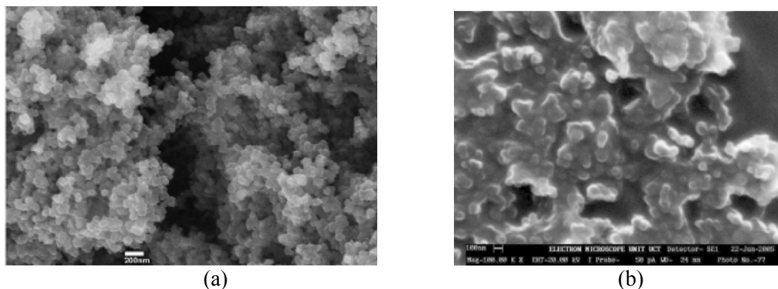
Figure 2.7. (a) a-Si:H nanoparticles as produced in a Hot-wire CVD process developed by Britton. (b) Nanoparticles as applied in ink jet printing process for the solar cell of Figure 5. [Hot-wire synthesis of Si nanoparticles Scriba MR, Arendse C, Härting M, Britton DT, Thin Solid Films 516 844-846 (2008).]
