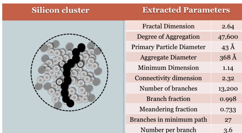
Figure 2.5. Results of USAX analysis using University of Cincinnati instrument and printed silicon electronics from the group of Britton and Härting (2010).
