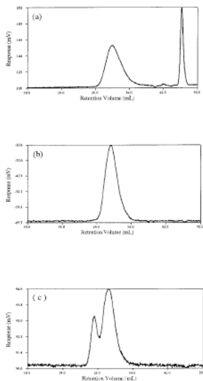
Figure 9. Response versus retention volume for a) RID, b) VD and c) LS detector for the same sample [66].
