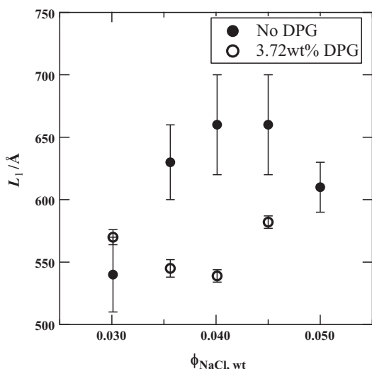
Fig. 4. Kuhn length, L_1 , versus weight fraction salt, \phi_{\text{NaCl, wt}} , with and without DPG showing a decrease in persistence in the presence of DPG.
