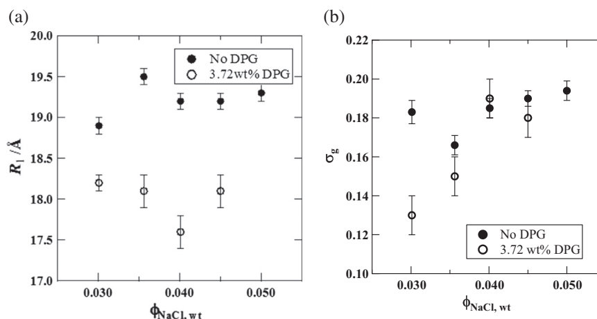
Fig. 3. (a) WLM/ellipsoid radius, R_1 , as a function of weight fraction salt (b) Dimensionless geometric standard deviation, \sigma_g , of the log-normal distribution for the cylindrical radius as a function of weight fraction salt.
