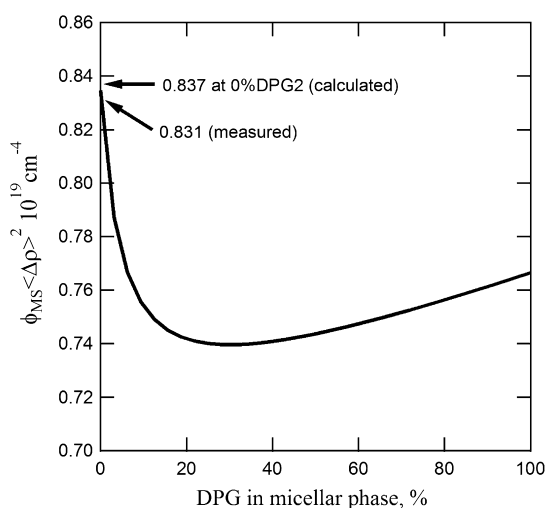
Fig. 2. Calculated scattering contrast ( \phi_{MS}(\Delta\rho)^2 ) versus percentage of DPG participating in the micellar phase. Solid line is calculated from Eq. (5).
