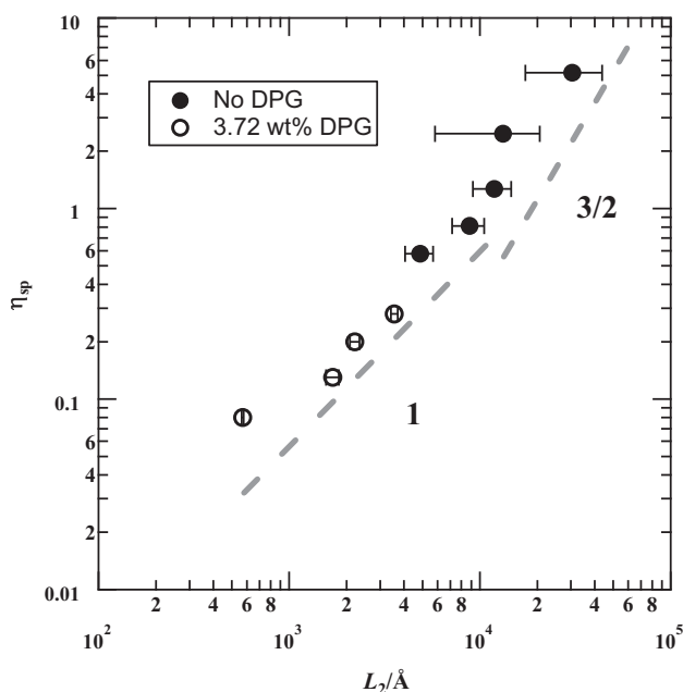
Fig. 6. Plot of \eta_{sp} versus L_2 showing different power law dependence for 0% and 3.72% DPG respectively.
