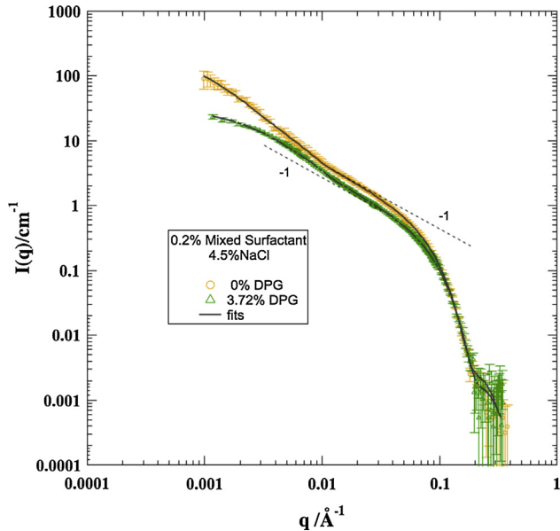
Fig. 1. Log-log plot of scattered intensity, I(q) , versus scattering vector, q . Low- q corresponds to large sizes and the difference in intensity in this region reflects a reduction in contour length for the DPG samples, 0.001 – 0.006 \text{ Å}^{-1} . Between 0.04 and 0.1 \text{ Å}^{-1} , the difference between the curves reflects a slightly smaller WLM radius in the presence of DPG. The region indicated by the -1 power-law slope reflects the cylindrical Kuhn structure. Deviation from this -1 power-law at low- q indicates the presence of a convoluted WLM structure. (Complete data and fits from this study are given in the supplemental material .)
