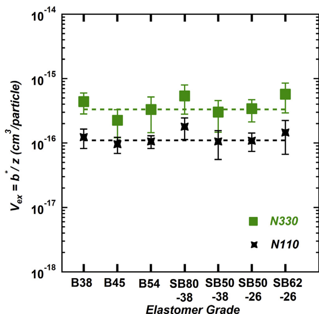
Fig. 7. Terminal state of dispersion characterized by the excluded volume b^* normalized by the degree of aggregation as a function of different elastomer grades for both carbon blacks – N110 (black stars) and N330 (green squares). The dashed horizontal lines indicate the average V_{ex} for each carbon black over all elastomer grades. (For interpretation of the references to colour in this figure legend, the reader is referred to the Web version of this article.)
