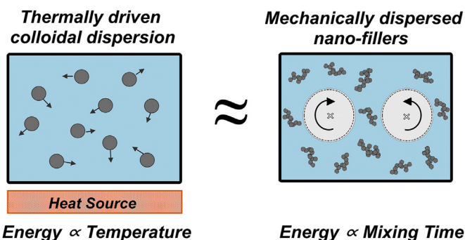
Fig. 2. A cartoon depicting the thermally-dispersed, colloidal analogy for mechanically mixed rubber-carbon black nanocomposites. The figure on the left shows colloidal particles in a solution where the average energy possessed by the particles is proportional to the temperature, T of the medium. The figure on the right shows carbon black aggregates in a rubber medium. The average kinetic energy is proportional to the total mixing time, t .
