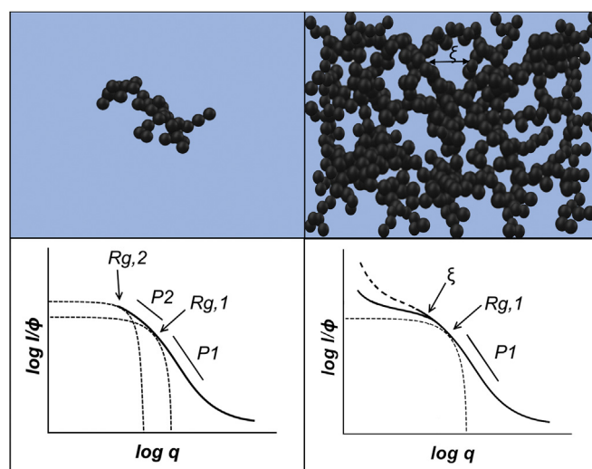
Fig. 1. (a) Cartoon of smallest dispersible unit (filler aggregate) with the corresponding scattering curve under dilute conditions. The filler exhibits a hierarchical structure and the scattering curve resolves each structural level as a power law slope ( P_1 , P_2 ) that gives information about the shape and a knee region that provides the size ( R_{g,1} , R_{g,2} ) of that level. (b) Cartoon indicating filler aggregate screening characterized by loss of structural resolution at large sizes for high concentrations, the corresponding scattering curve translates this loss in structural features as loss of reduced intensity at the aggregate level compared to the dilute scattering profile.
