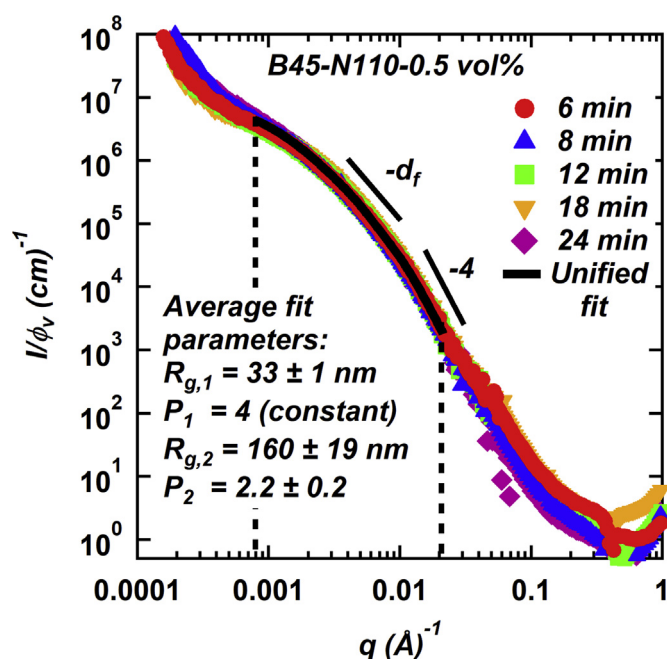
Fig. 3. Dilute USAXS curves for 0.5 vol percent B45-N110 nanocomposites milled at different processing times. The q -range between the dashed lines used to analyze the carbon black structure corresponds to level 1 (primary particle) and level 2 (aggregate) of the structural hierarchy; USAXS curves for dilute (0.5 vol percent) B45-N330 nanocomposites are shown in Fig. S1 in the supplemental material.
