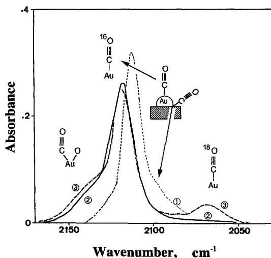
Fig. 5. IR absorption spectra in the carbonyl stretching region produced by different interactions. Curve 1, 0.5 mbar of ^{16}\text{CO} ; curve 2, inlet of 0.5 mbar of ^{16}\text{O}_2 ; curve 3, inlet of 0.5 mbar of ^{18}\text{O}_2 .
