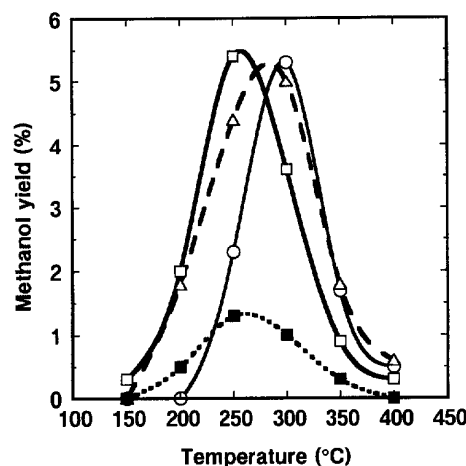
Fig. 7. Methanol yield as a function of reaction temperature in the hydrogenation of CO 2 over supported gold catalysts. ○, Au/ZnO (Au/Zn = 1:19); □, Au/α-Fe 2 O 3 (Au/Fe = 1:19); Δ, Cu/ZnO (Cu/Zn = 1:19); ■, Au/TiO 2 (Au/Ti = 1:19). CO 2 /H 2 /Ar = 23:67:10, 50 atm, SV = 3000 ml/h per g-cat.
