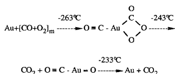
Scheme 1. Reactivity of atomic gold.
