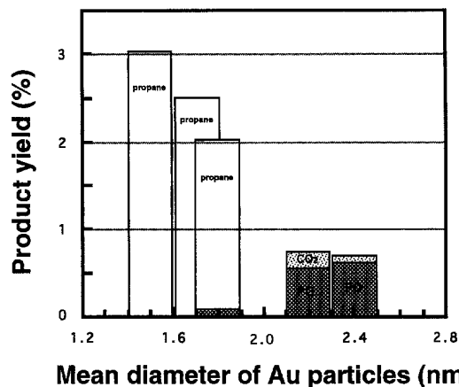
Fig. 6. Product yields for the reaction of propylene with O 2 and H 2 over Au/TiO 2 catalysts as a function of the mean diameters of Au particles. Feed gas, H 2 /O 2 /propylene/Ar (10:10:10:70, vol%); space velocity 4000 ml/h per g-cat.; reaction temperature 80°C.
