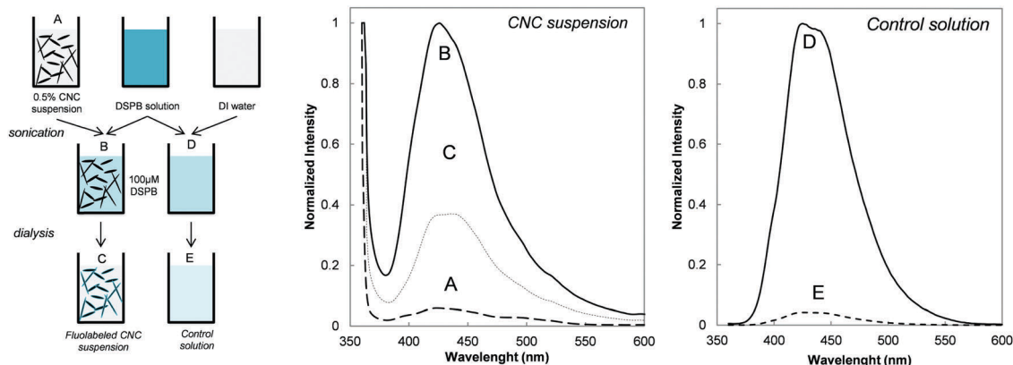
Fig. 33 Fluorescence spectra of 0.5 wt% neat CNC suspension (A), with 100 \mu\text{M} DSBP solution before (B) and after dialysis (C). Control spectra corresponding to the 100 \mu\text{M} DSBP solution before (D) and after dialysis (E). Intensities are standardized with respect to the absorbance of a 100 \mu\text{M} DSBP solution. \lambda_{\text{ex}} = 351 nm. Reprinted from ref. 342. Reproduced with permission from Romanian Academy Publishing House, the owner of the publishing rights.
