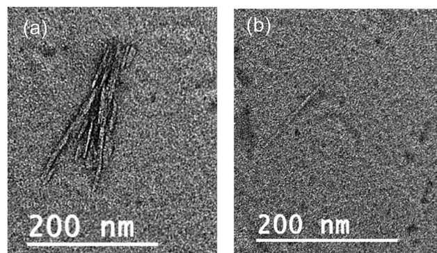
Fig. 21 TEM images of CNCs prepared with (a) negative staining and (b) unstained (both images taken around 100k \times magnification). Unpublished images courtesy of Foster, Roberts and Stinson-Bagby.
