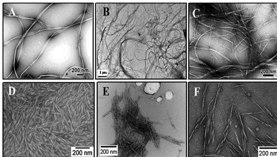
Fig. 23 TEM images of CNCs obtained from (A) bacterial cellulose CNFs, (B) bagasse CNFs, (C) banana rachis CNFs, (D) rice straw CNCs, (E) soy hulls CNCs, (F) mengkuang leave CNCs. Reprinted by permission from ref. 46, copyright Springer.
